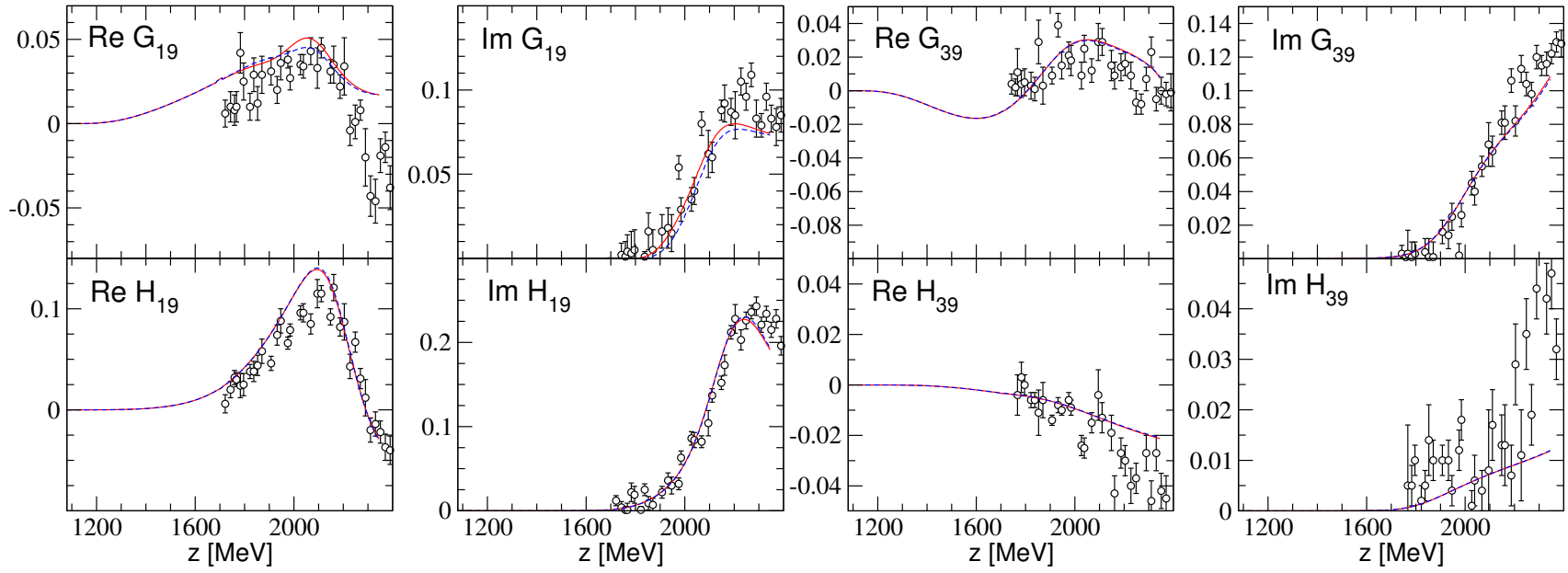
Figure 3: JüBo_omegaN: red (solid) line for fit A, blue (dashed) line for fit B. Points: GWU-SAID WI08 solution (Phys. Rev. C 86, 035202 (2012)).
