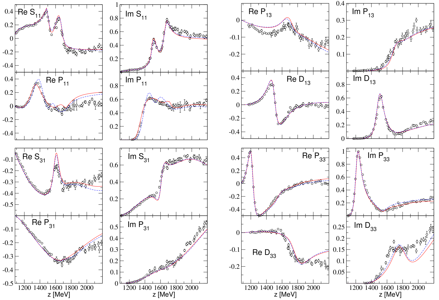
Figure 1: JüBo_omegaN: red (solid) line for fit A, blue (dashed) line for fit B. Points: GWU-SAID WI08 solution (Phys. Rev. C 86, 035202 (2012)).
