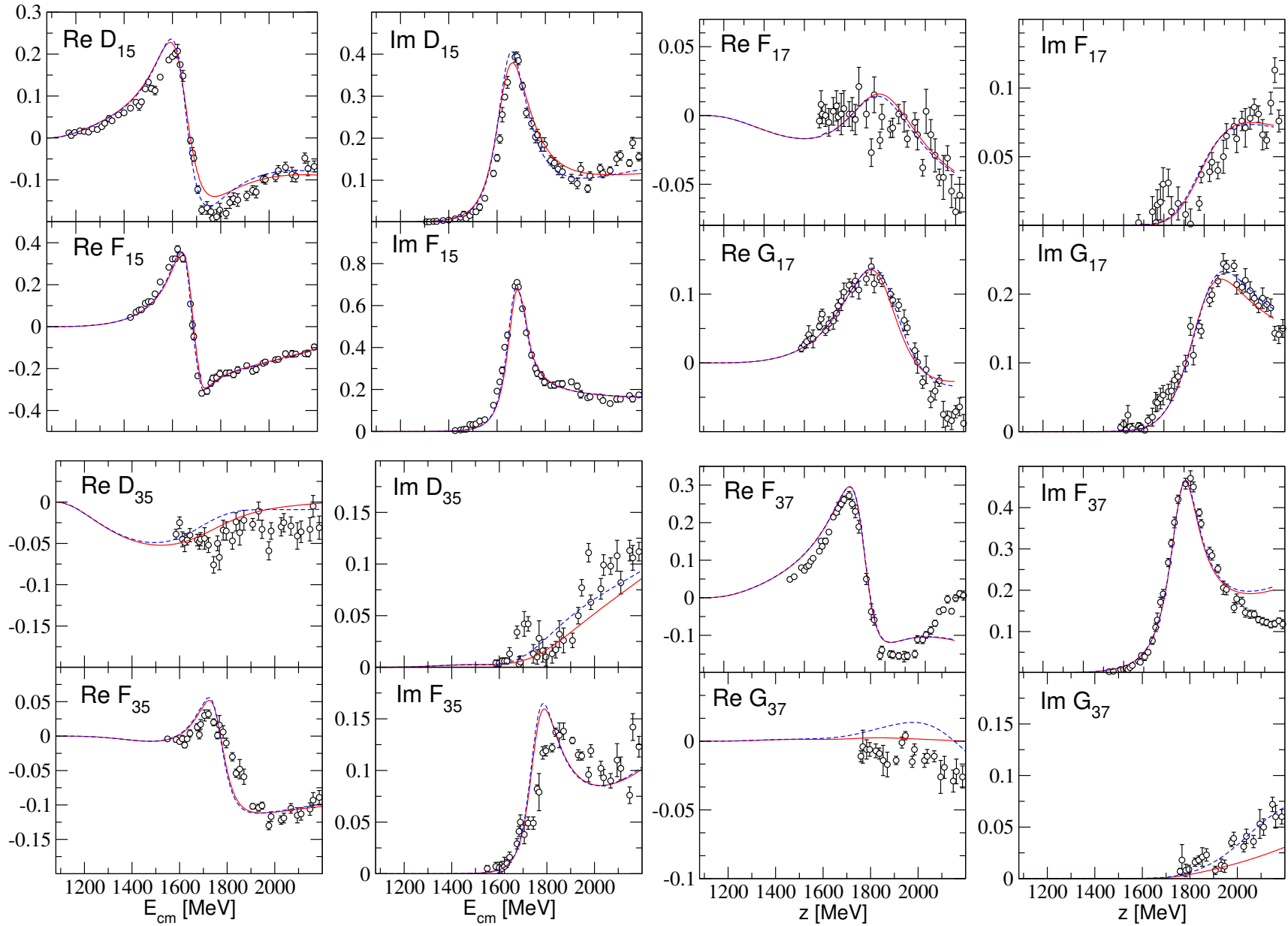
Figure 2: JüBo_omegaN: red (solid) line for fit A, blue (dashed) line for fit B. Points: GWU-SAID WI08 solution (Phys. Rev. C 86, 035202 (2012)).
