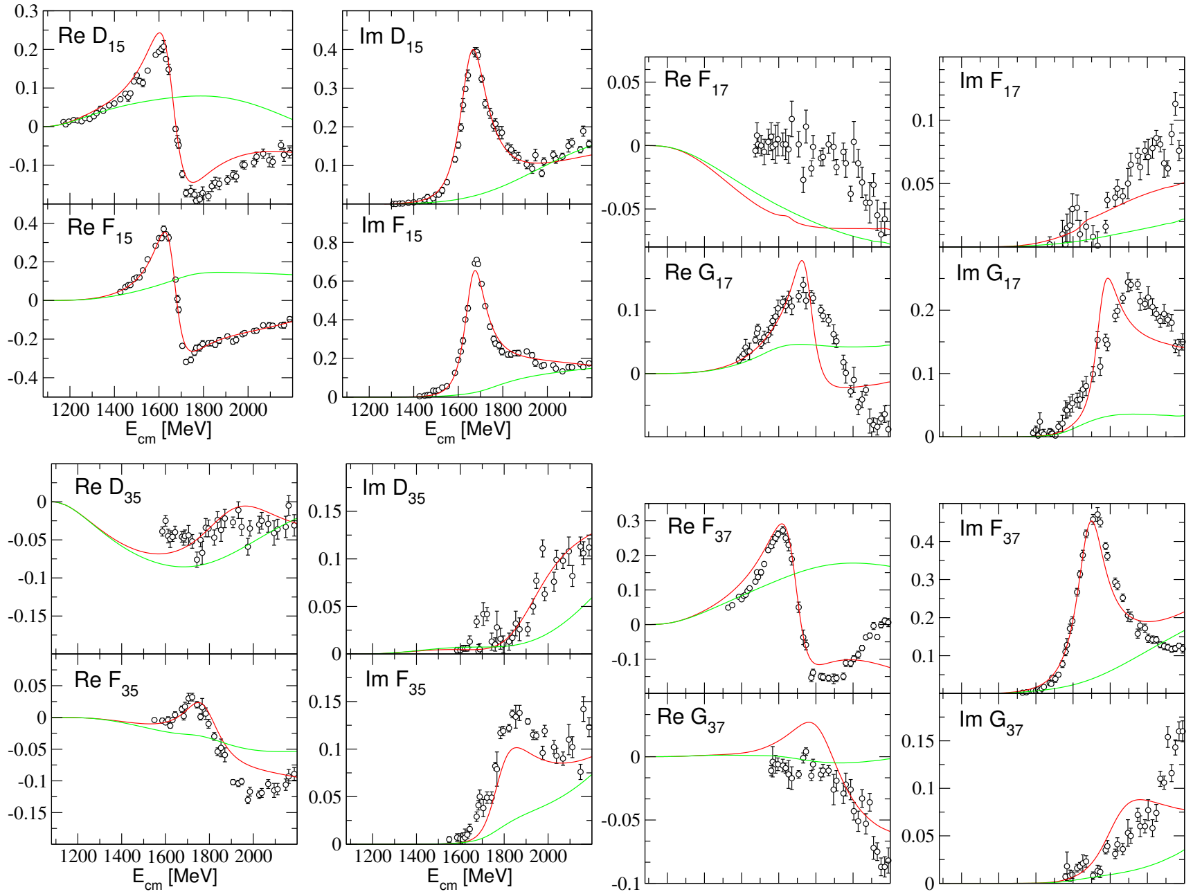
Figure 2: JüBo2025: red (solid) line, T^{\text{NP}} : green line. Points: GWU-SAID WI08 solution (Phys. Rev. C 86, 035202 (2012)).
