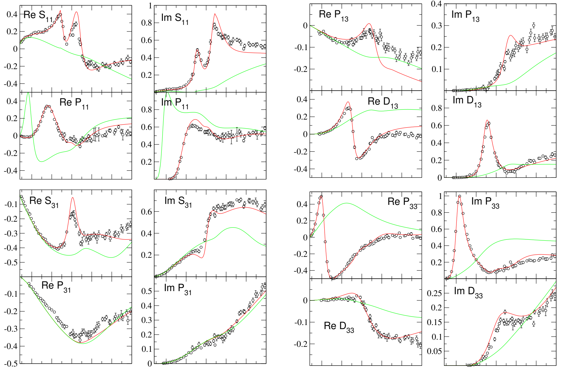
Figure 1: JüBo2025: red (solid) line, T^{\text{NP}} : green line. Points: GWU-SAID WI08 solution (Phys. Rev. C 86, 035202 (2012)).
