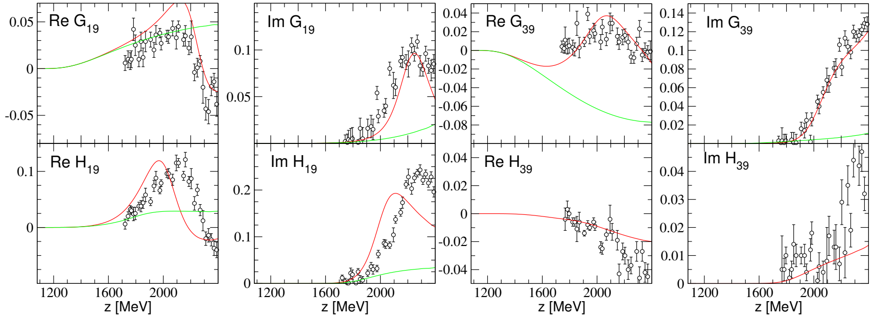
Figure 3: JüBo2025: red (solid) line, T^{\text{NP}} : green line. Points: GWU-SAID WI08 solution (Phys. Rev. C 86, 035202 (2012)).
