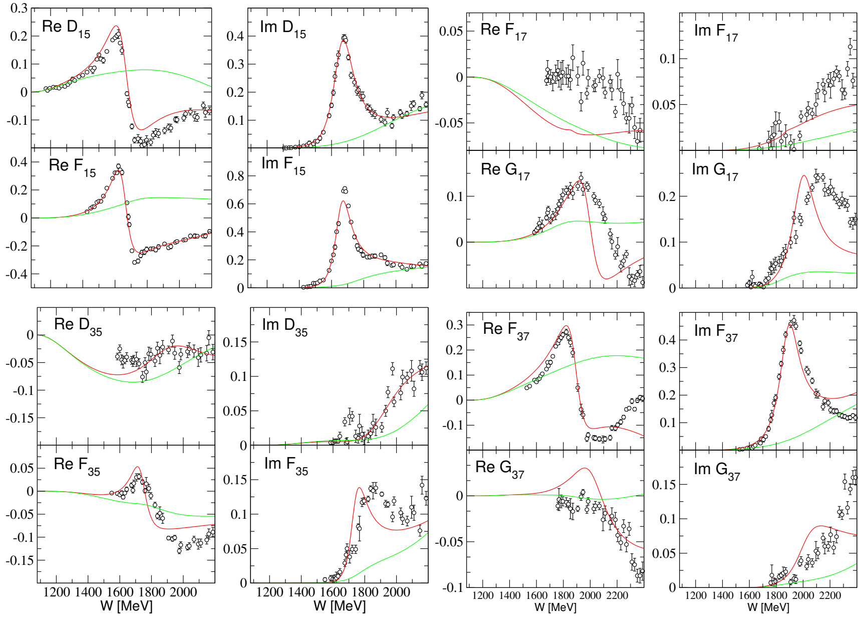
Figure 2: JüBo2022: red (solid) line, T^{\text{NP}} : green line. Points: GWU-SAID WI08 solution (Phys. Rev. C 86, 035202 (2012)).
