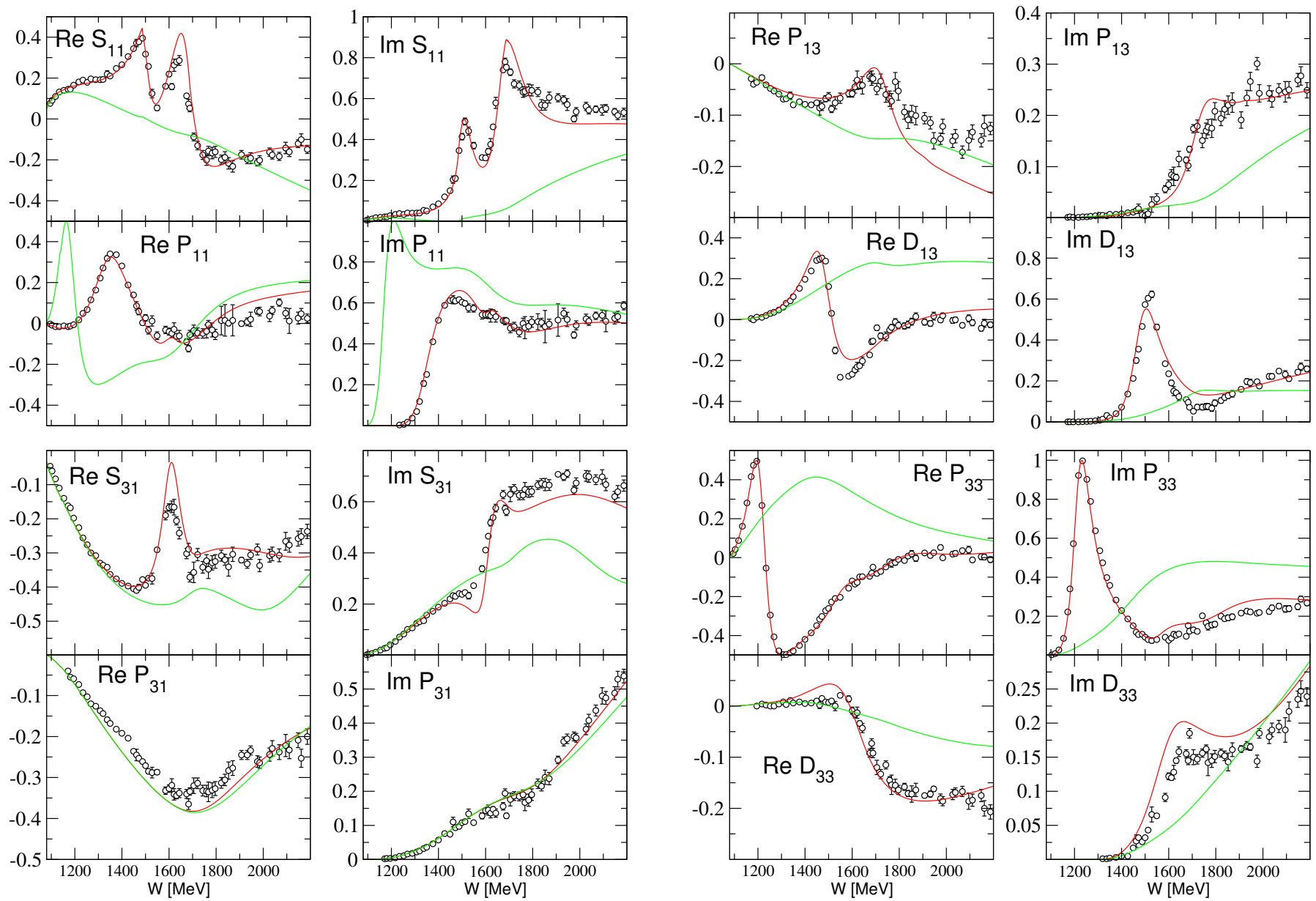
Figure 1: JüBo2022: red (solid) line, T^{\text{NP}} : green line. Points: GWU-SAID WI08 solution (Phys. Rev. C 86, 035202 (2012)).
