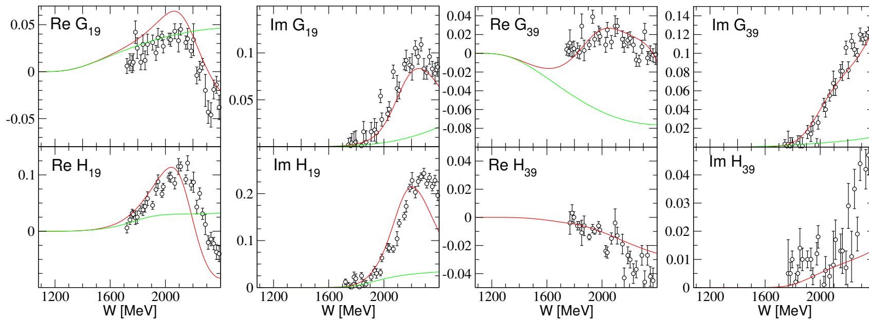
Figure 3: JüBo2022: red (solid) line, T^{\text{NP}} : green line. Points: GWU-SAID WI08 solution (Phys. Rev. C 86, 035202 (2012)).
