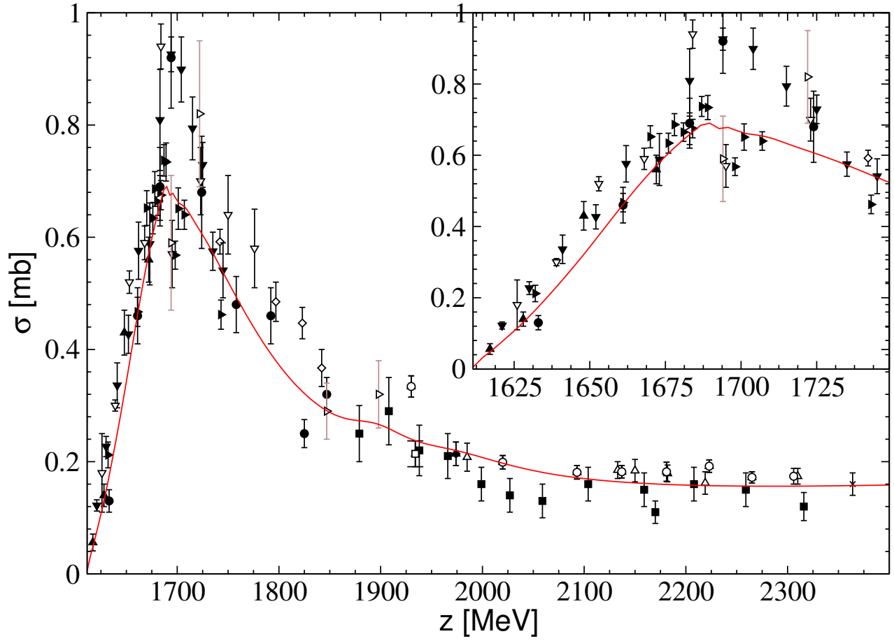
Figure 7: Total cross section of the reaction \pi^- p \rightarrow K^0 \Lambda . Data: filled circles from Ref. [12]; filled squares from Ref. [13]; empty diamonds from Ref. [14]; empty triangles up from Ref. [15]; filled triangles up from Ref. [16]; filled triangles down from Ref. [21]; empty triangles down from Ref. [22]; filled triangles right from Ref. [17]; empty triangles left from Ref. [23]; empty triangles right from Ref. [24]; empty squares from Ref. [18]; filled diamonds from Ref. [19]; stars from Ref. [25]; for empty circles and crosses see Ref. [26].
