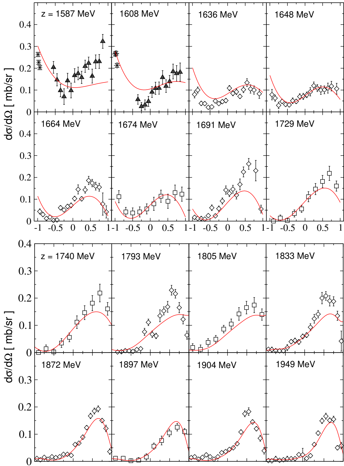
Figure 3: Differential cross section [2/3] of the reaction \pi^- p \rightarrow \eta n . Data: c.f. Fig. 2 and empty diamonds from Ref. [10].
