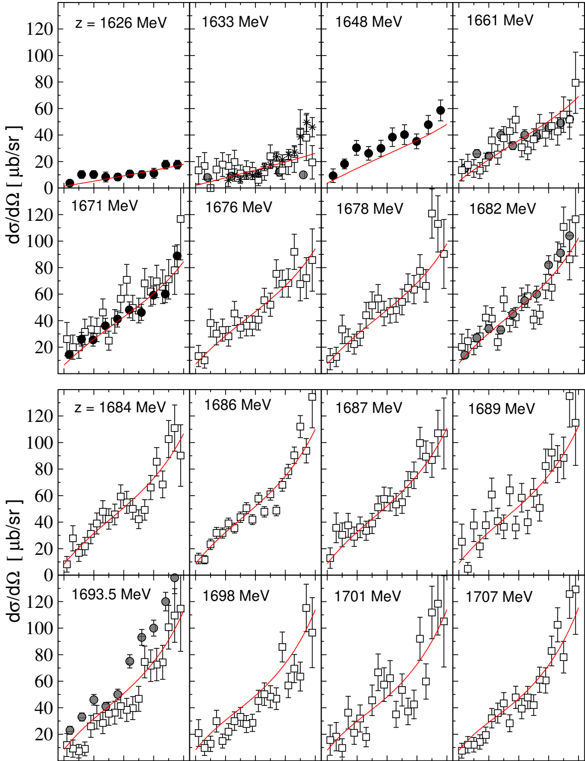
Figure 8: Differential cross section [1/3] of the reaction \pi^- p \rightarrow K^0 \Lambda . Data: filled circles from Ref. [16]; empty squares from Ref. [17]; partially filled circles from Ref. [12]; stars from Ref. [18]; triangles from Ref. [14]; empty diamonds from Ref. [13]; partially filled squares from Ref. [15]; filled diamonds from Ref. [19].
