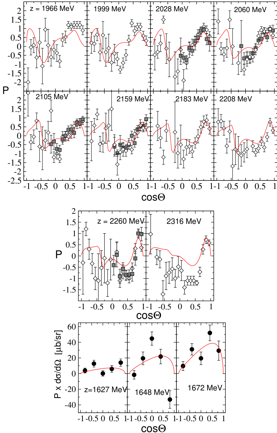
Figure 12: Polarization [2/2] of the reaction \pi^- p \rightarrow K^0 \Lambda . Data: c.f Fig. 11.
