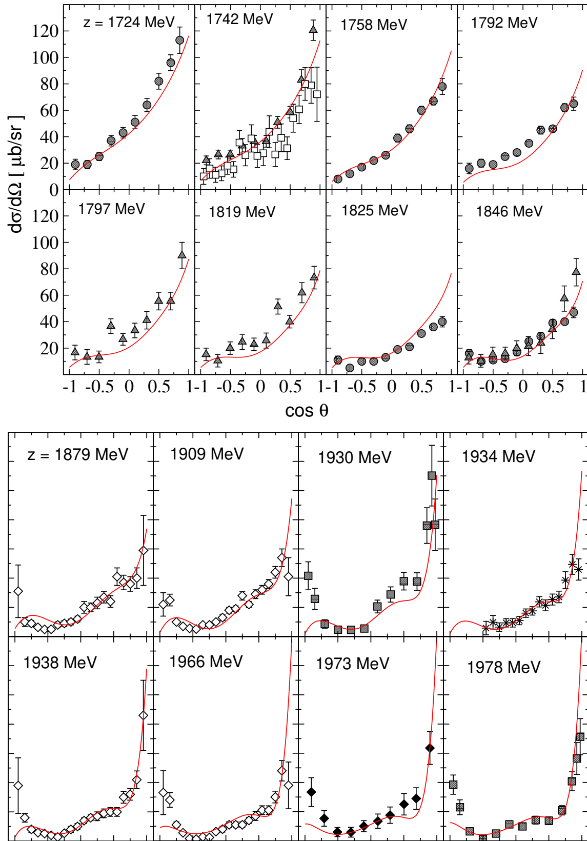
Figure 9: Differential cross section [2/3] of the reaction \pi^- p \rightarrow K^0 \Lambda . Data: c.f. Fig. 8.
