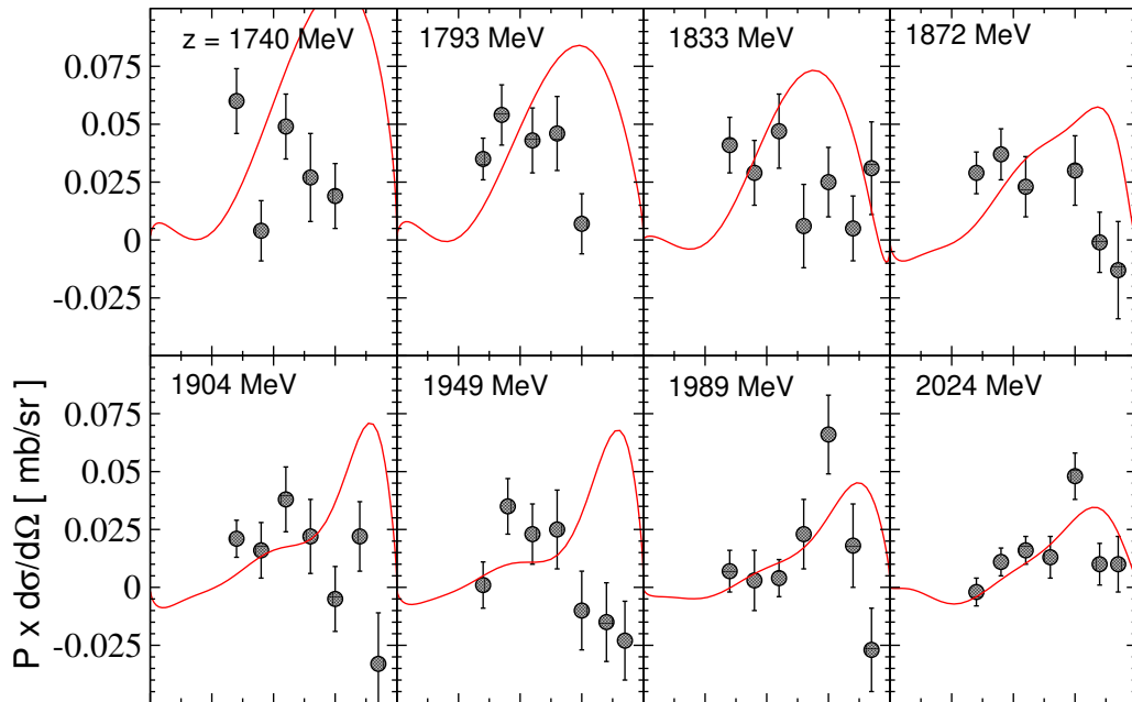
Figure 5: Polarization [1/2] of the reaction \pi^- p \rightarrow \eta n . Data: Ref. [11].
