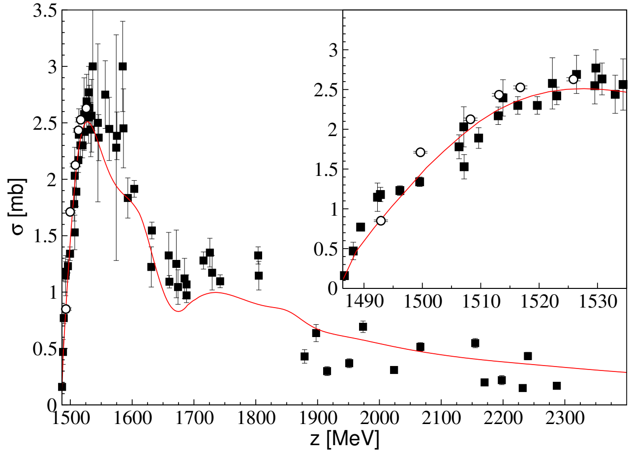
Figure 1: Total cross section of the reaction \pi^- p \rightarrow \eta n . Data: the filled squares indicate experiments accepted by the GWU/SAID group [1]; open circles from Ref. [2].
