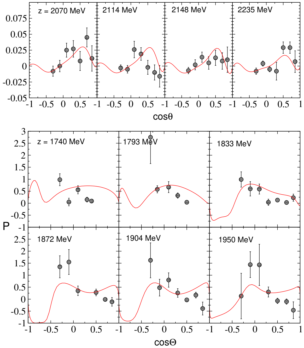
Figure 6: Polarization [2/2] of the reaction \pi^- p \rightarrow \eta n . Data: Ref. [11].
