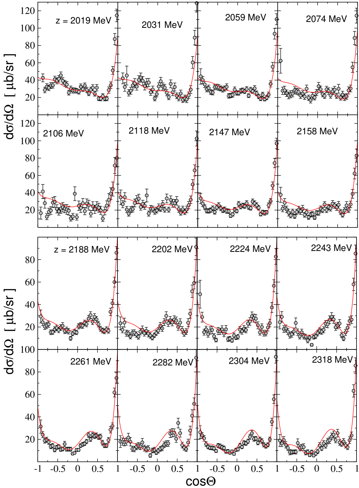
Figure 22: Differential cross section [2/2] of the reaction \pi^+p \rightarrow K^+\Sigma^+ . Data from Ref. [35].
