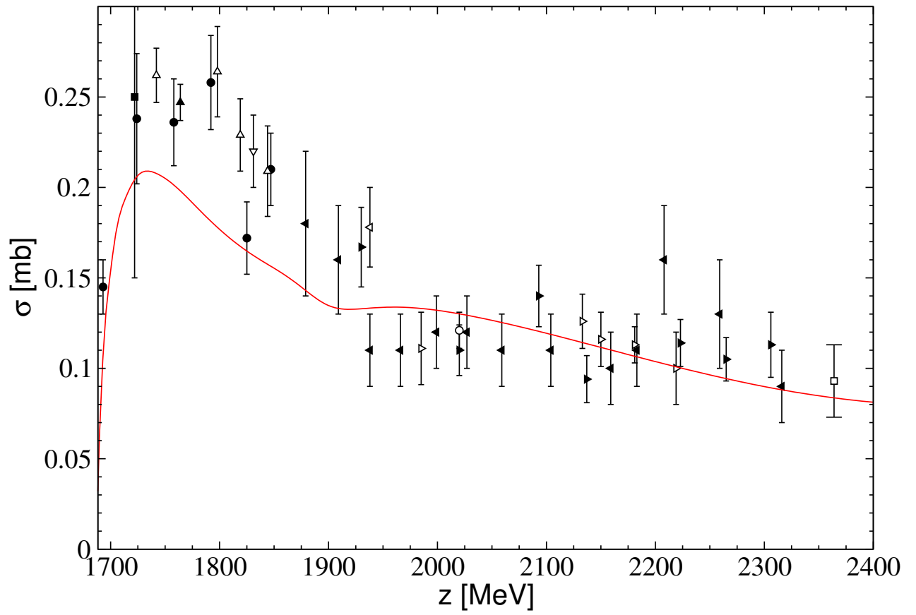
Figure 14: Total cross section of the reaction \pi^- p \rightarrow K^0 \Sigma^0 . Data: empty triangles up: Ref. [14]; empty triangles right: Ref. [15]; filled squares: Ref. [24]; empty triangles left: Ref. [19]; filled triangles up: Ref. [29] filled circles: Ref. [27]; empty circles: Ref. [30]; filled triangles left: Ref. [28]. For empty triangles down, filled triangles right, and empty squares see [26].
