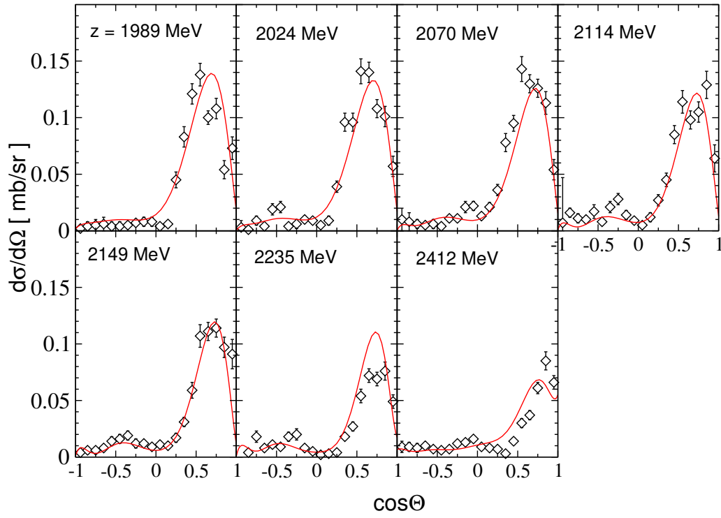
Figure 4: Differential cross section [3/3] of the reaction \pi^- p \rightarrow \eta n . Data: c.f. Fig. 3.
