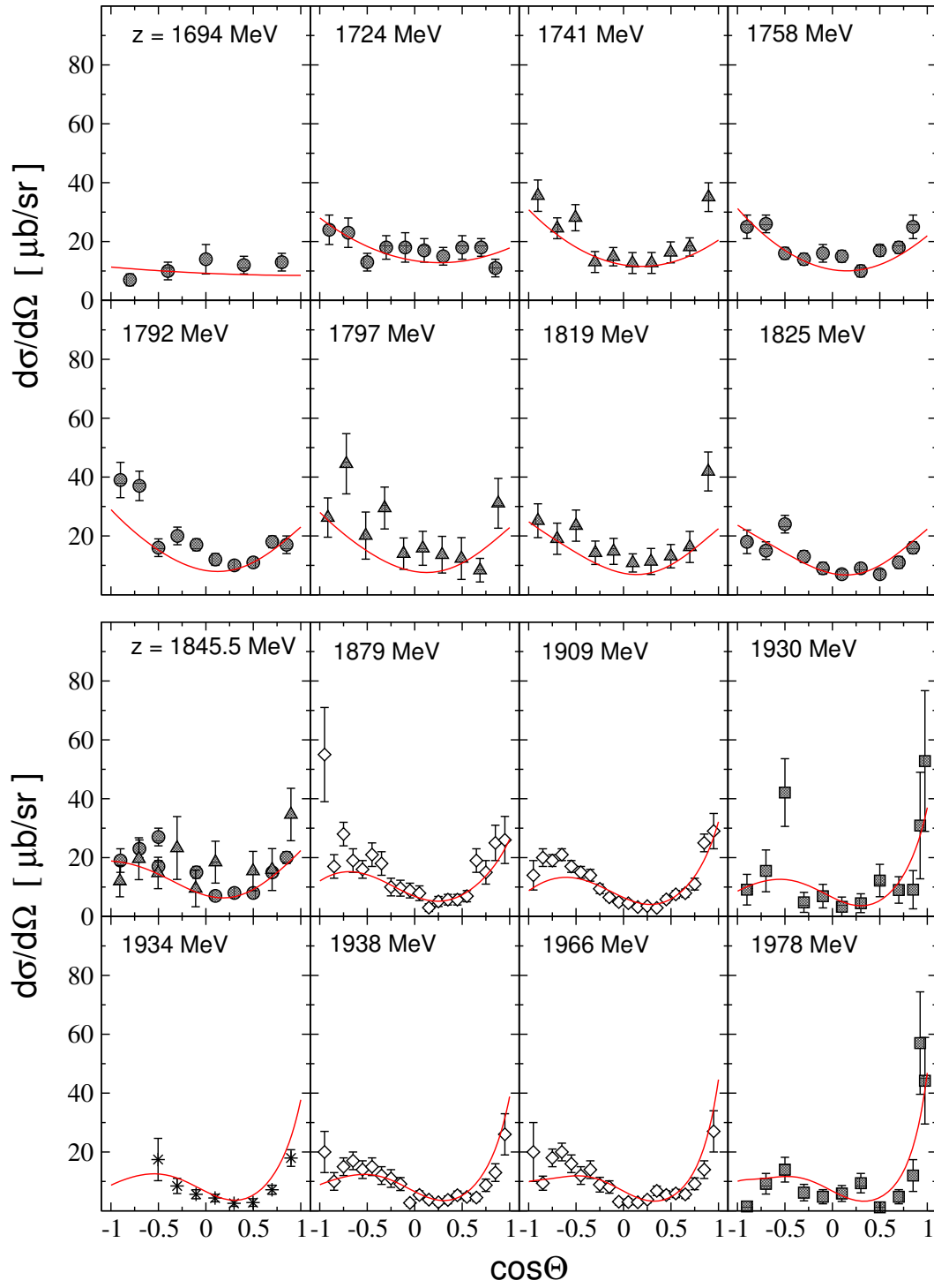
Figure 15: Differential cross section [1/2] of the reaction \pi^- p \rightarrow K^0 \Sigma^0 . Data: circles from Ref. [27]; up triangles from Ref. [14]; squares from Ref. [15]; diamonds from Ref. [28]; stars from Ref. [18].
