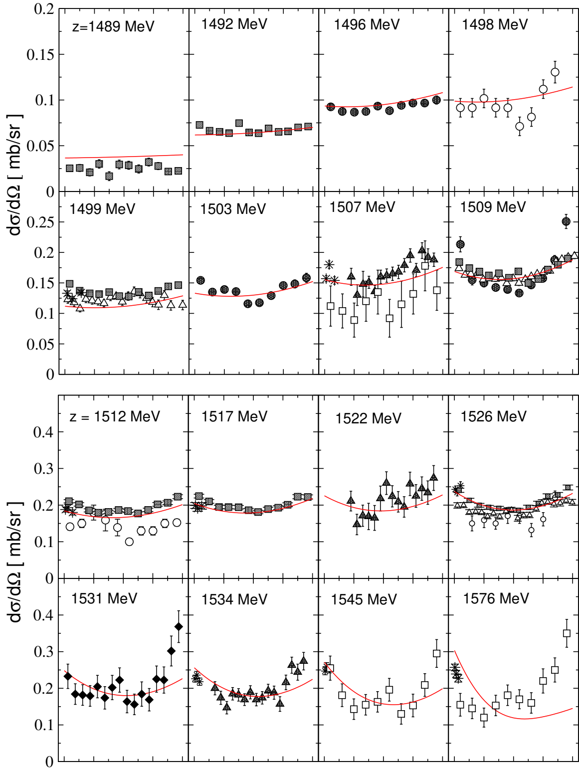
Figure 2: Differential cross section [1/3] of the reaction \pi^- p \rightarrow \eta n . Data: filled squares from Ref. [2]; filled circles from Ref. [3]; empty circles from Ref. [4]; empty triangles up from Ref. [5]; stars from Ref. [6]; filled triangles up from Ref. [7]; empty squares from Ref. [8]; filled diamonds from Ref. [9].
