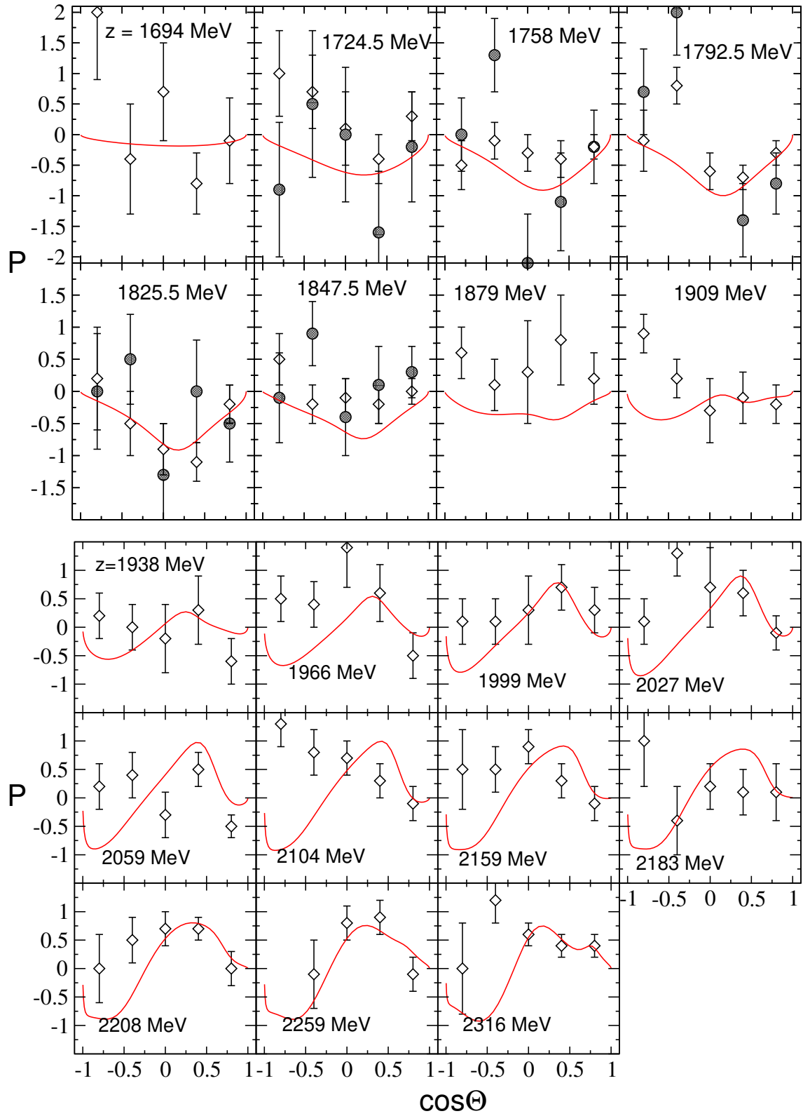
Figure 17: Polarization of the reaction \pi^- p \rightarrow K^0 \Sigma^0 . Data: circles from Ref. [27]; diamonds from Ref. [28].
