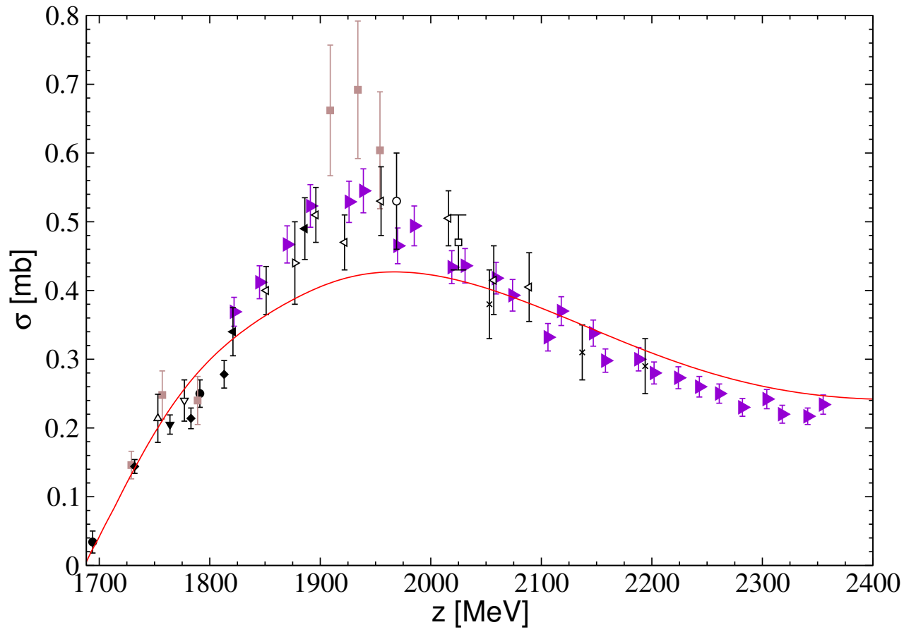
Figure 20: Total cross section of the reaction \pi^+p \rightarrow K^+\Sigma^+ . Data: filled triangles right: Ref. [35]; filled squares: Ref. [40]; filled diamonds: Ref. [41]; empty triangles up: Ref. [47]; filled triangles down: Ref. [43]; empty triangles down: Ref. [48]; empty triangles left: Ref. [49]; empty circles: Ref. [50]; empty squares: Ref. [51]; crosses: Ref. [52]. For filled circles, filled triangles left and empty triangles right see Ref. [26].
