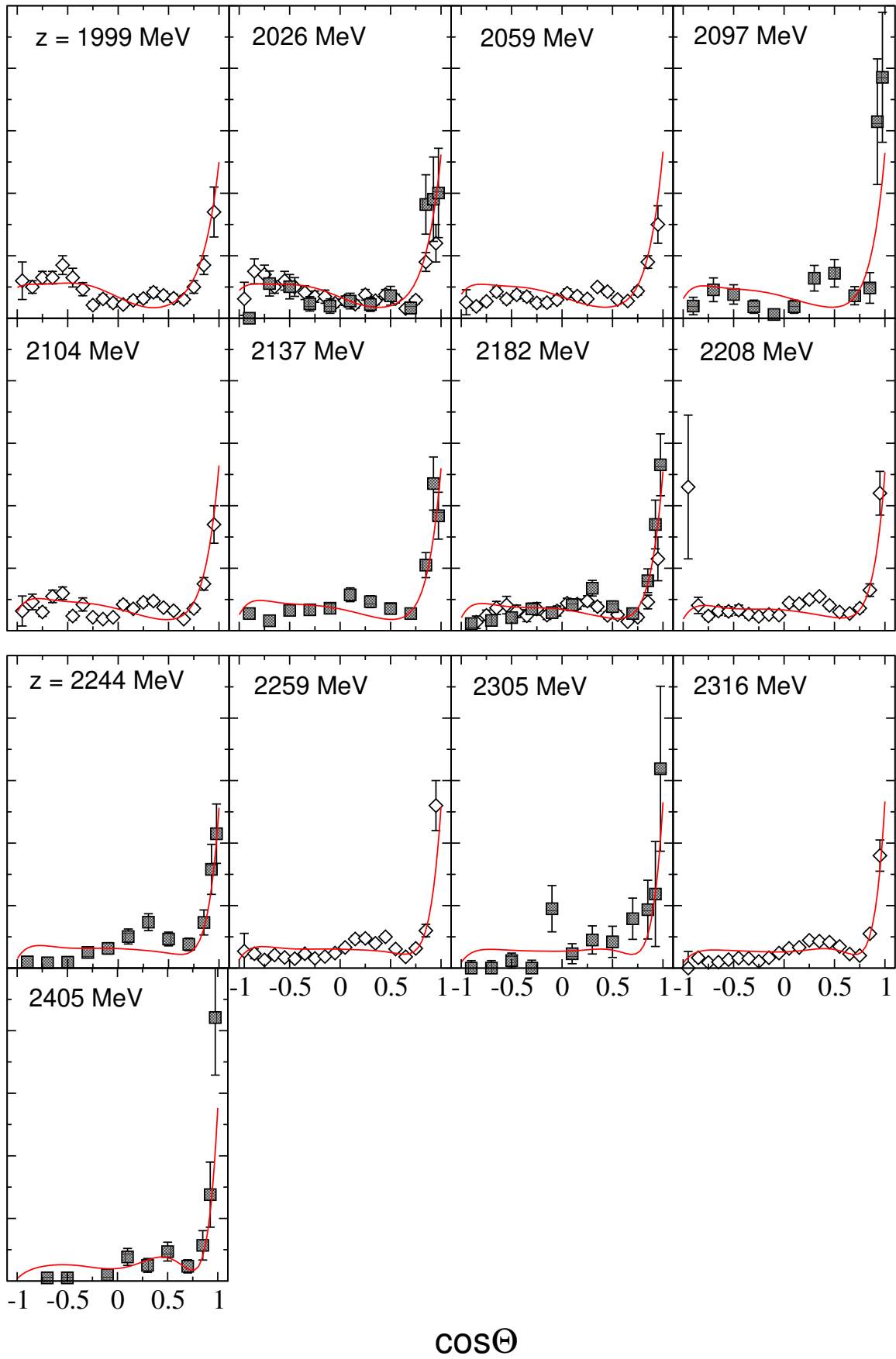
Figure 16: Differential cross section [2/2] of the reaction \pi^- p \rightarrow K^0 \Sigma^0 . Data: c.f. Fig. 15.
