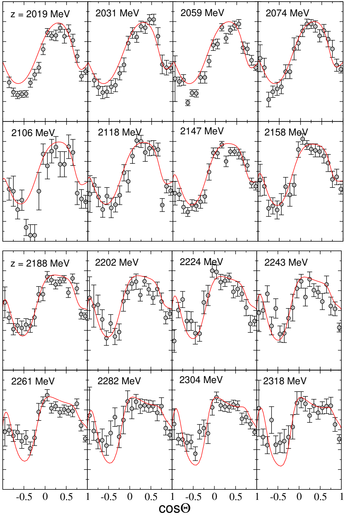
Figure 24: Polarization [2/2] of the reaction \pi^+p \rightarrow K^+\Sigma^+ . Data: Ref. [35].
