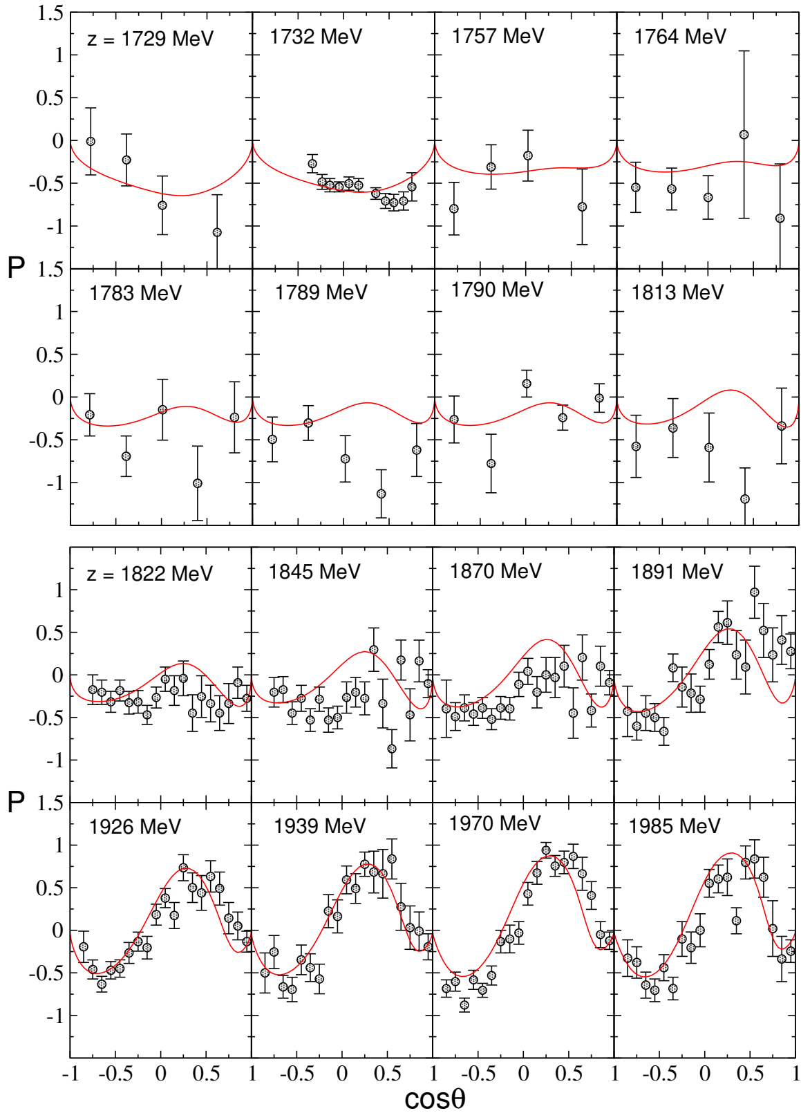
Figure 23: Polarization [1/2] of the reaction \pi^+p \rightarrow K^+\Sigma^+ . Data: Ref. [35], except: z = 1729, 1757, 1789 MeV from Ref. [40]; z = 1783, 1813 MeV from Ref. [41]; z = 1764 MeV from Ref. [43]; z = 1790 MeV from Ref. [42]; z = 1732 MeV from Ref. [44].
