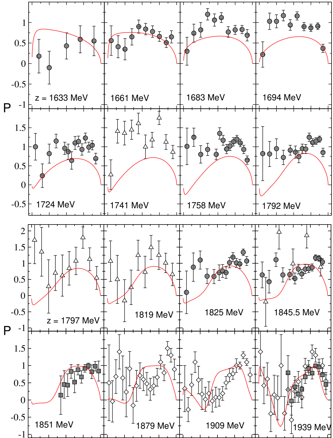
Figure 11: Polarization [1/2] of the reaction \pi^- p \rightarrow K^0 \Lambda . Data: filled circles from Ref. [12]; empty triangles up from Ref. [14]; filled squares from Ref. [20]; empty diamonds from Ref. [13].
