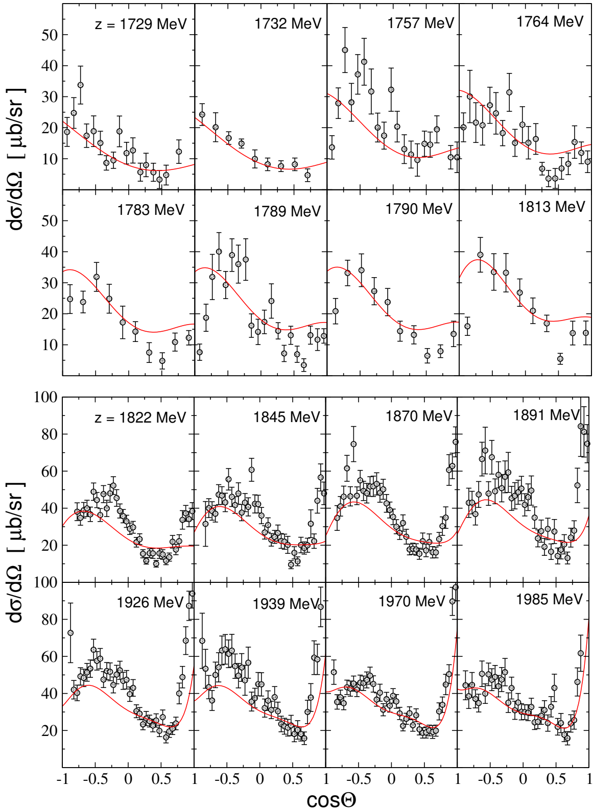
Figure 21: Differential cross section [1/2] of the reaction \pi^+p \rightarrow K^+\Sigma^+ . Data: Ref. [35], except: z = 1729, 1757, 1789 MeV from Ref. [40]; z = 1732, 1783, 1813 MeV from Ref. [41]; z = 1764 MeV from Ref. [43]; z = 1790 MeV from Ref. [42].
