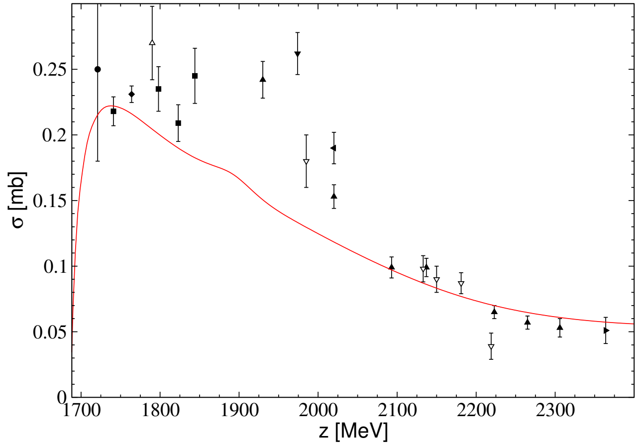
Figure 18: Total cross section of the reaction \pi^- p \rightarrow K^+ \Sigma^- . Data: empty triangles down: Ref. [15]; filled circles: Ref. [24]; filled triangles down: Ref. [19]; filled triangles left: Ref. [30]; empty triangles up: Ref. [34]; filled squares: Ref. [32]; filled diamonds: Ref. [33]. For filled triangles up and filled triangles right see Ref. [26].
