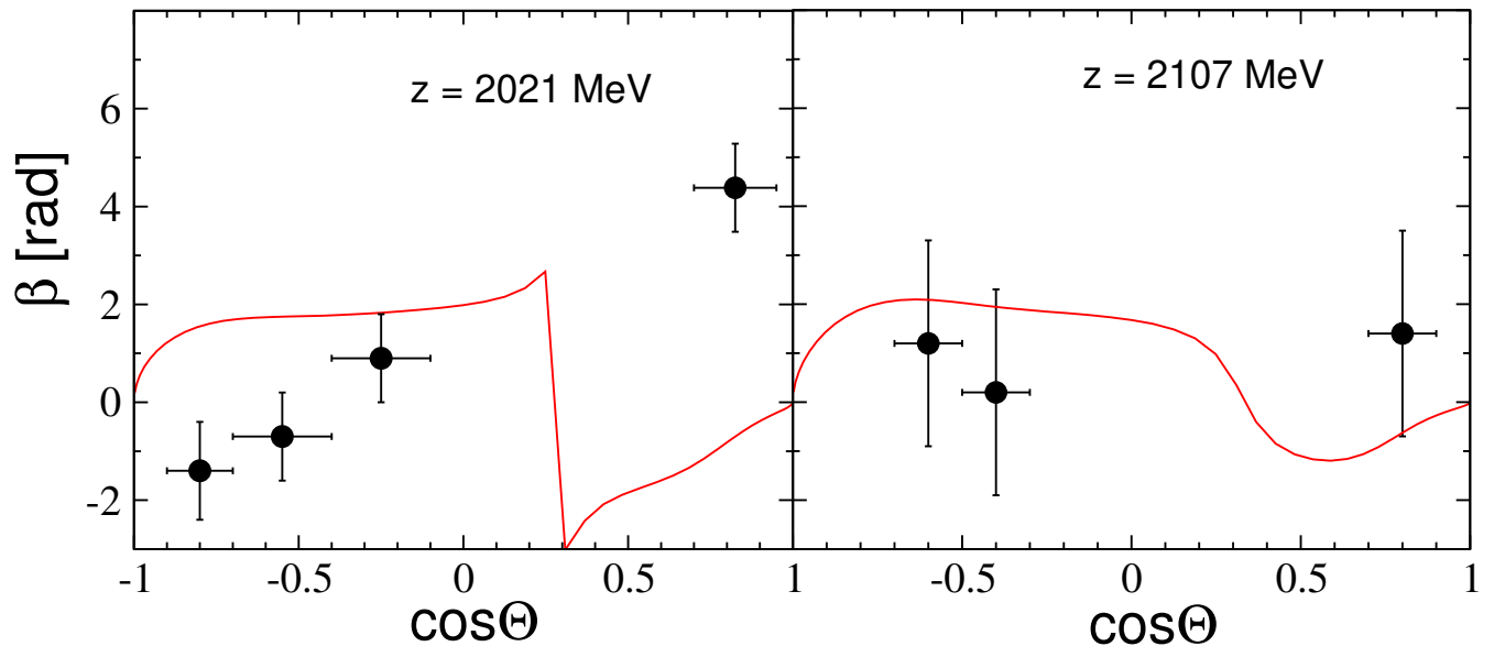
Figure 25: Spin-rotation parameter \beta of the reaction \pi^+p \rightarrow K^+\Sigma^+ . Data: Ref. [37].
