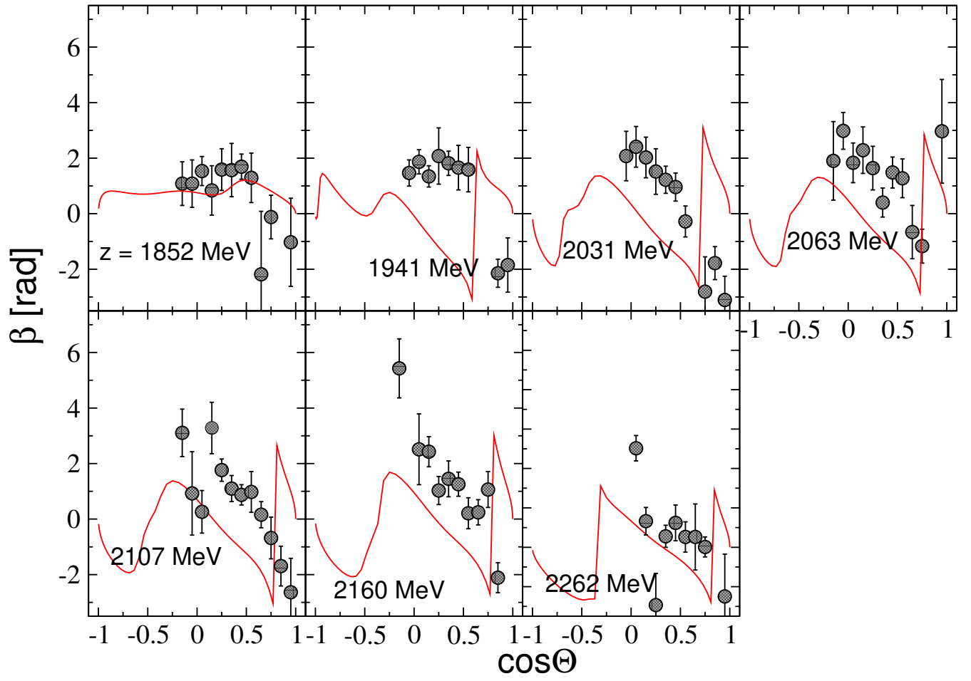
Figure 13: Spin-rotation parameter \beta of the reaction \pi^- p \rightarrow K^0 \Lambda . Data: Ref. [20].
