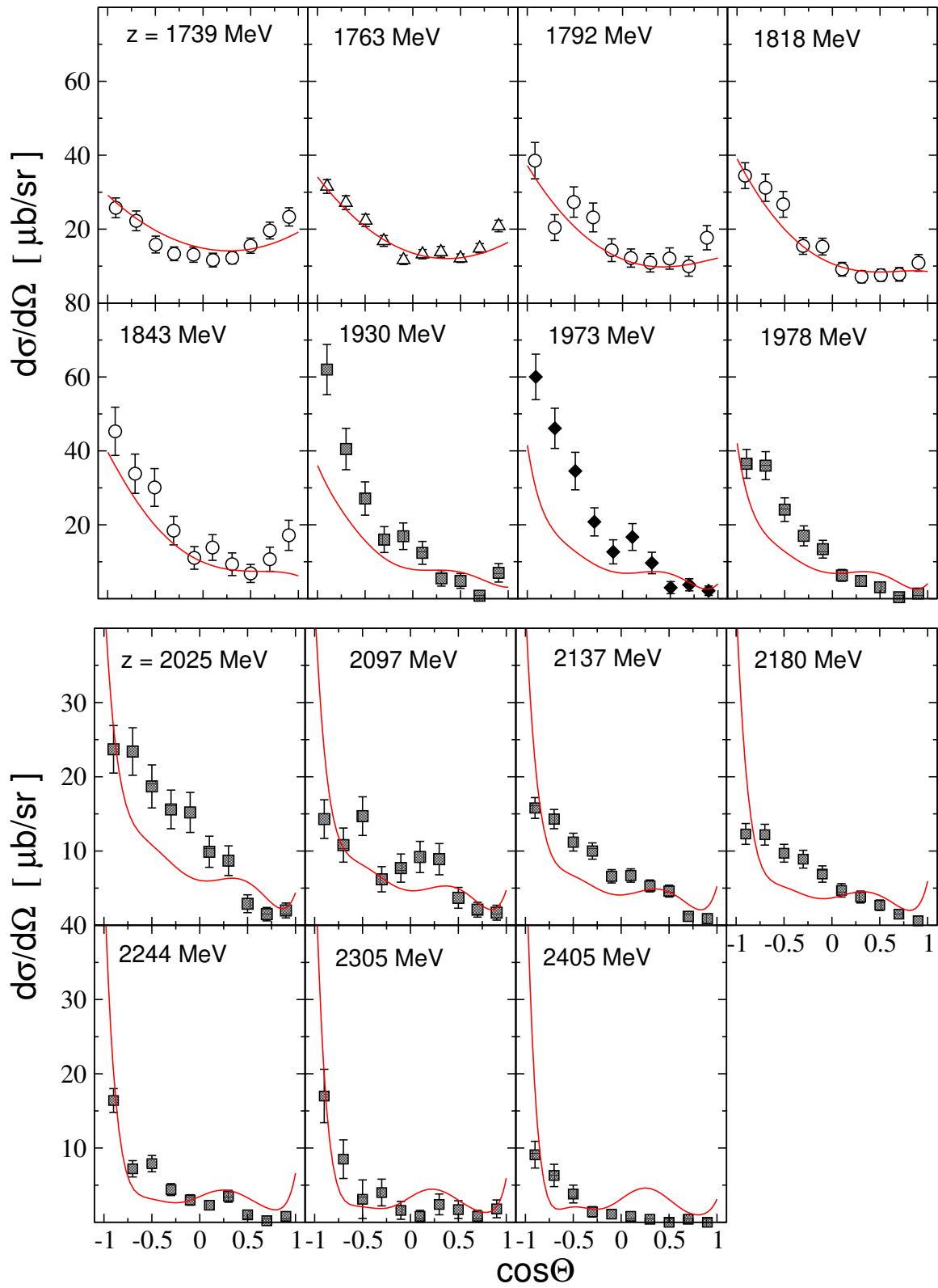
Figure 19: Differential cross section of the reaction \pi^- p \rightarrow K^+ \Sigma^- . Data: circles from Ref. [32]; up triangles from Ref. [33]; squares from Ref. [15]; diamonds from Ref. [19].
