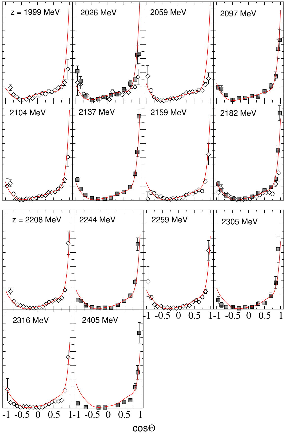
Figure 10: Differential cross section [3/3] of the reaction \pi^- p \rightarrow K^0 \Lambda . Data: c.f. Fig. 8.
