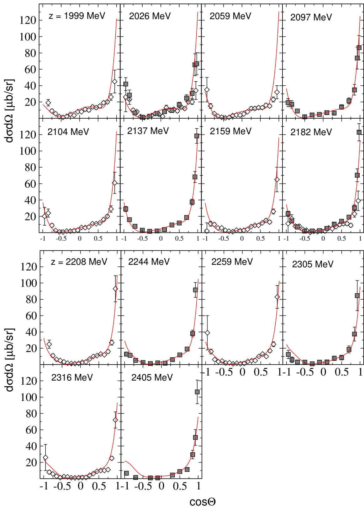
Figure 10: Differential cross section [3/3] of the reaction \pi^- p \rightarrow K^0 \Lambda . Data: c.f. Fig. 8.
