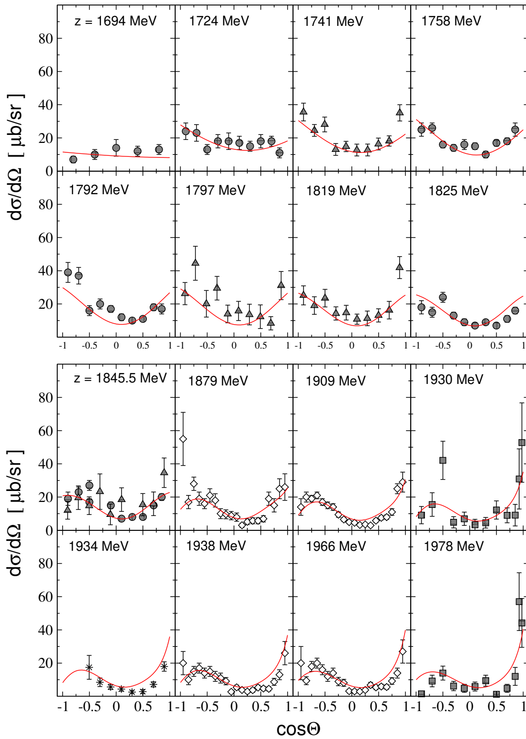
Figure 15: Differential cross section [1/2] of the reaction \pi^- p \rightarrow K^0 \Sigma^0 . Data: circles from Ref. [27]; up triangles from Ref. [14]; squares from Ref. [15]; diamonds from Ref. [28]; stars from Ref. [18].
