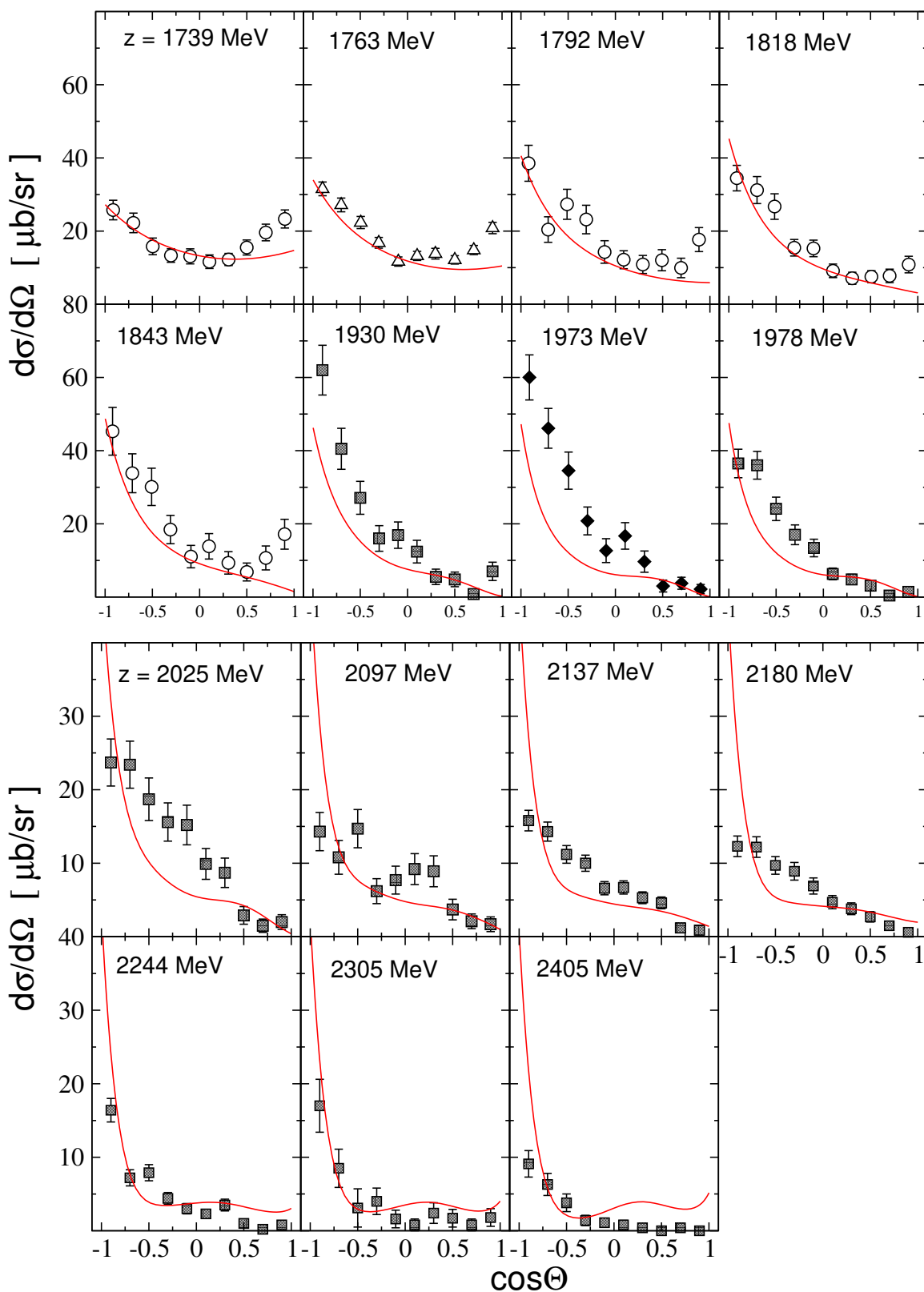
Figure 19: Differential cross section of the reaction \pi^- p \rightarrow K^+ \Sigma^- . Data: circles from Ref. [32]; up triangles from Ref. [33]; squares from Ref. [15]; diamonds from Ref. [19].
