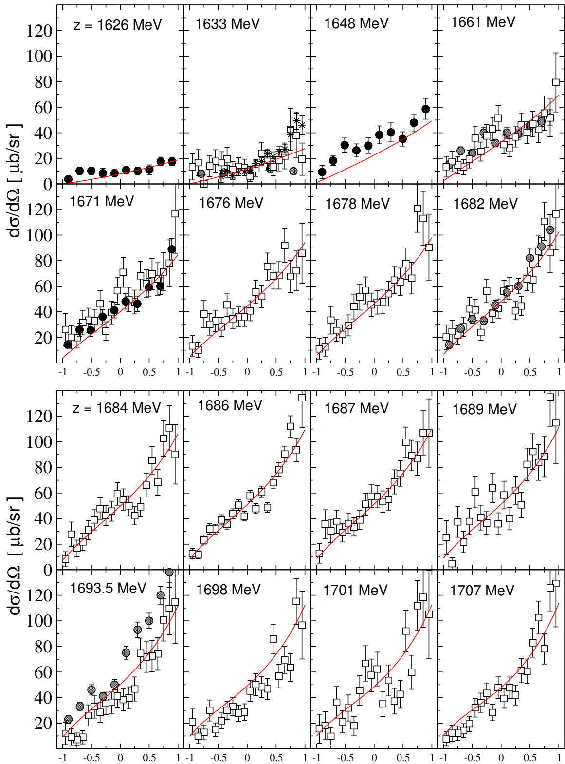
Figure 8: Differential cross section [1/3] of the reaction \pi^- p \rightarrow K^0 \Lambda . Data: filled circles from Ref. [16]; empty squares from Ref. [17]; partially filled circles from Ref. [12]; stars from Ref. [18]; triangles from Ref. [14]; empty diamonds from Ref. [13]; partially filled squares from Ref. [15]; filled diamonds from Ref. [19].
