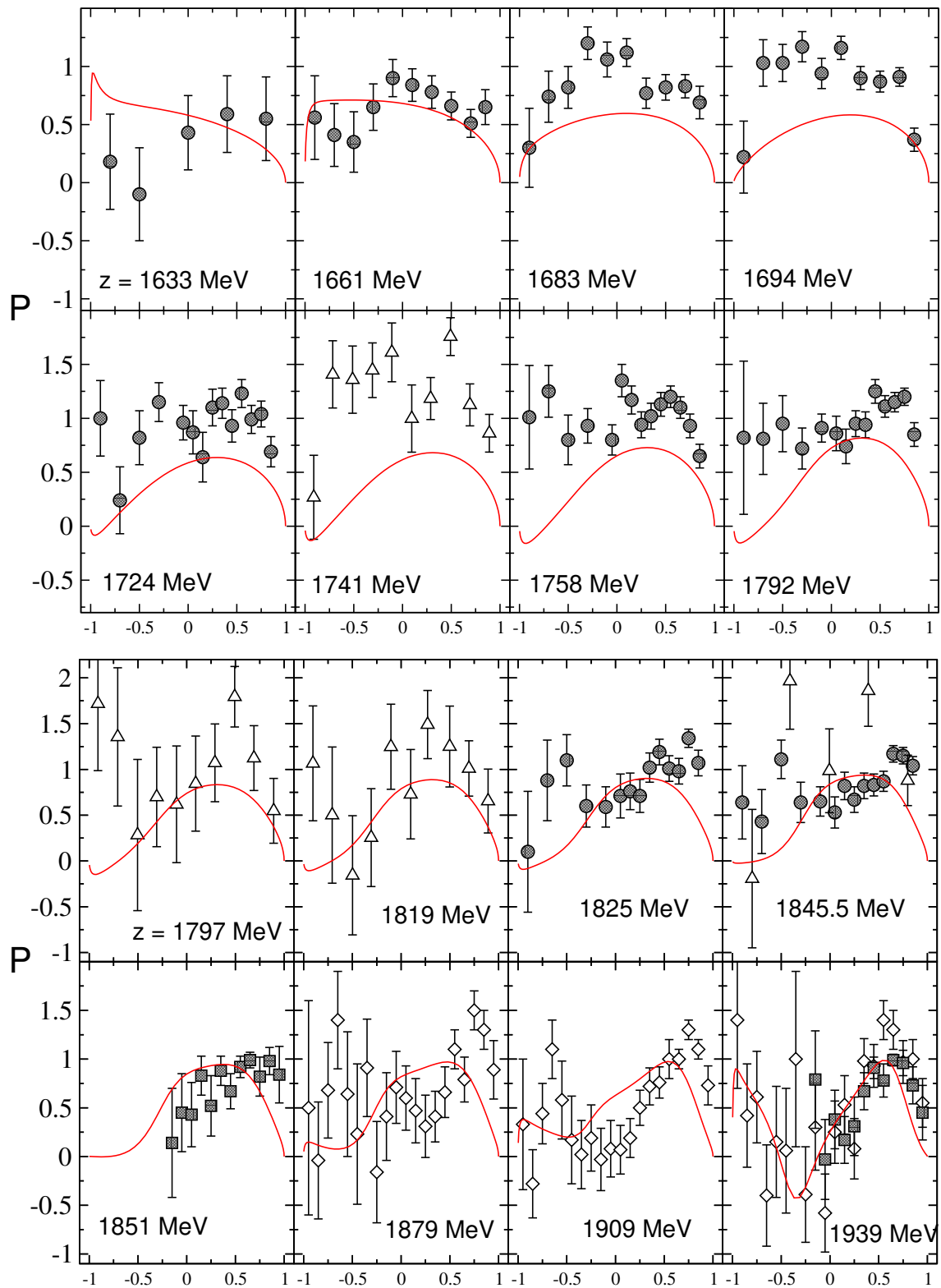
Figure 11: Polarization [1/2] of the reaction \pi^- p \rightarrow K^0 \Lambda . Data: filled circles from Ref. [12]; empty triangles up from Ref. [14]; filled squares from Ref. [20]; empty diamonds from Ref. [13].
