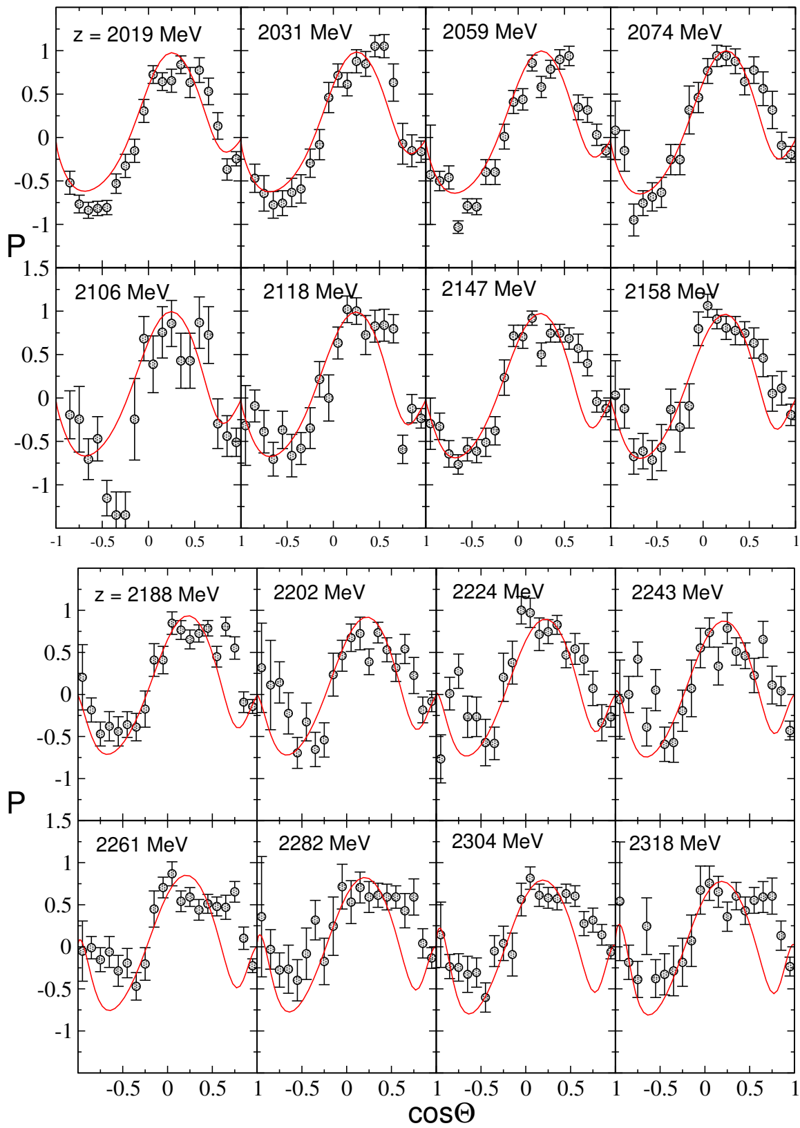
Figure 24: Polarization [2/2] of the reaction \pi^+p \rightarrow K^+\Sigma^+ . Data: Ref. [35].
