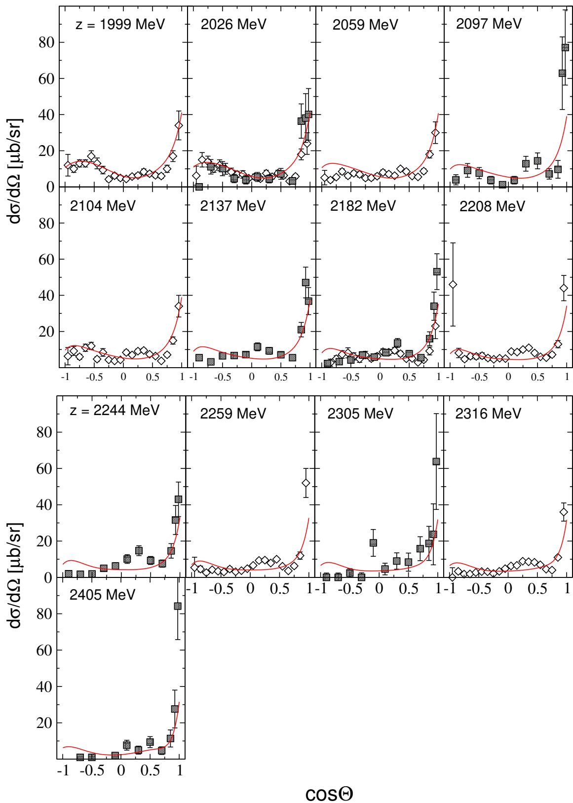
Figure 16: Differential cross section [2/2] of the reaction \pi^- p \rightarrow K^0 \Sigma^0 . Data: c.f. Fig. 15.
