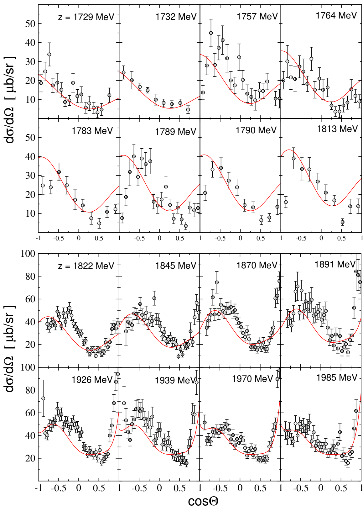
Figure 21: Differential cross section [1/2] of the reaction \pi^+p \rightarrow K^+\Sigma^+ . Data: Ref. [35], except: z = 1729, 1757, 1789 MeV from Ref. [40]; z = 1732, 1783, 1813 MeV from Ref. [41]; z = 1764 MeV from Ref. [43]; z = 1790 MeV from Ref. [42].
