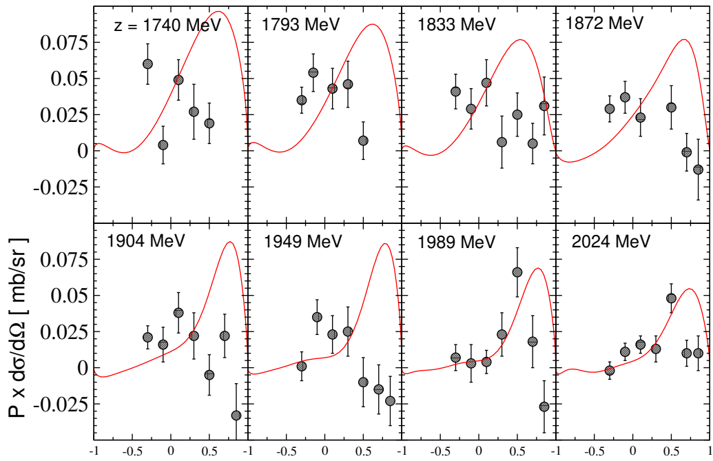
Figure 5: Polarization [1/2] of the reaction \pi^- p \rightarrow \eta n . Data: Ref. [11].
