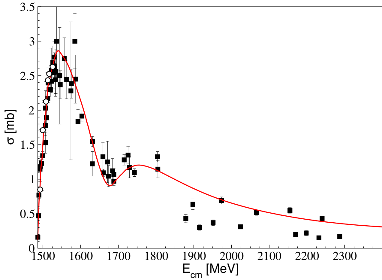
Figure 1: Total cross section of the reaction \pi^- p \rightarrow \eta n . Data: the filled squares indicate experiments accepted by the GWU/SAID group [1]; open circles from Ref. [2].
