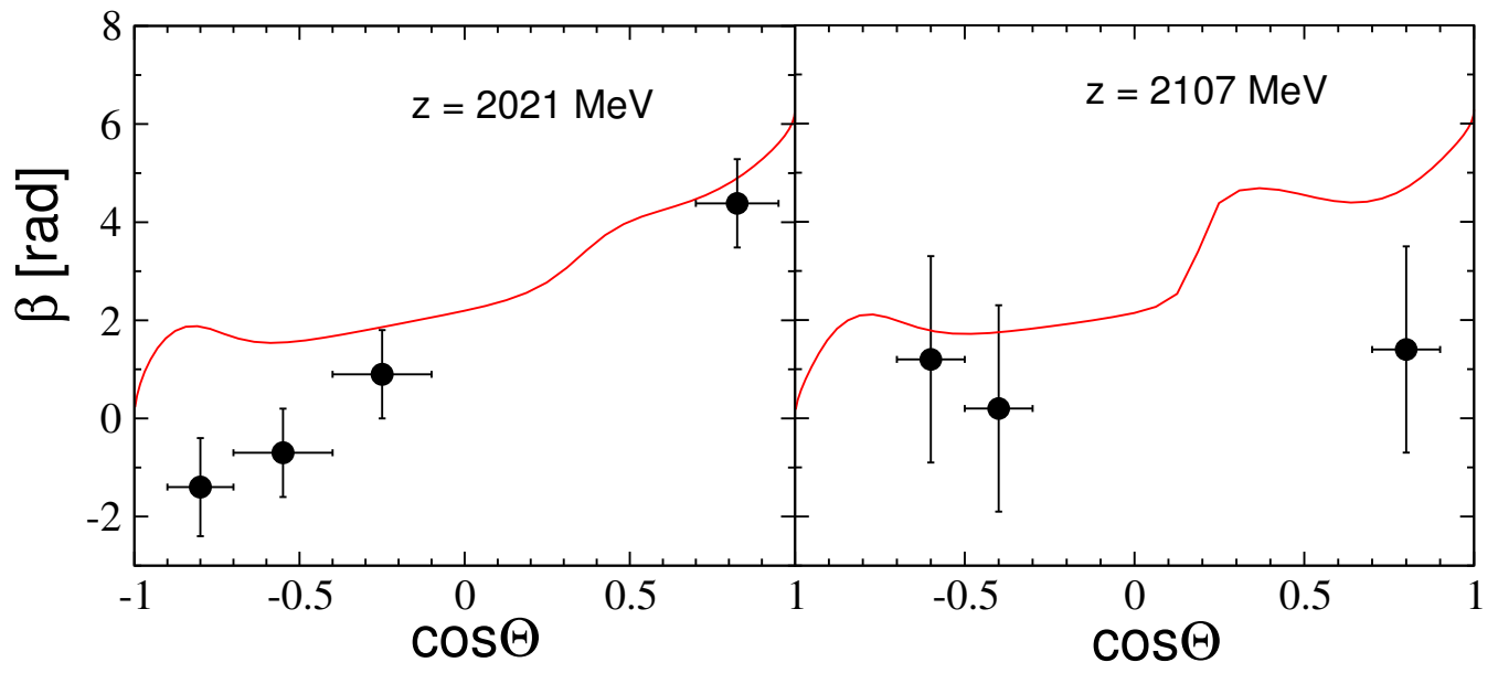
Figure 25: Spin-rotation parameter \beta of the reaction \pi^+p \rightarrow K^+\Sigma^+ . Data: Ref. [37].
