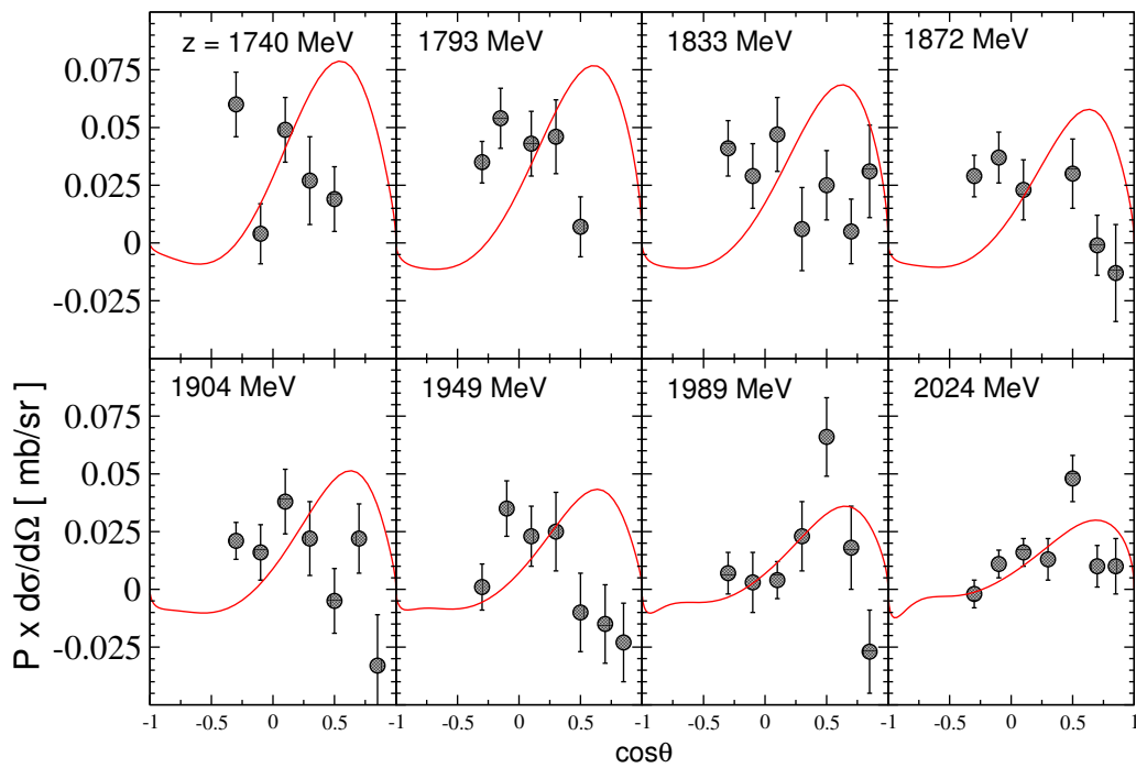
Figure 5: Polarization [1/2] of the reaction \pi^- p \rightarrow \eta n . Data: Ref. [11].
