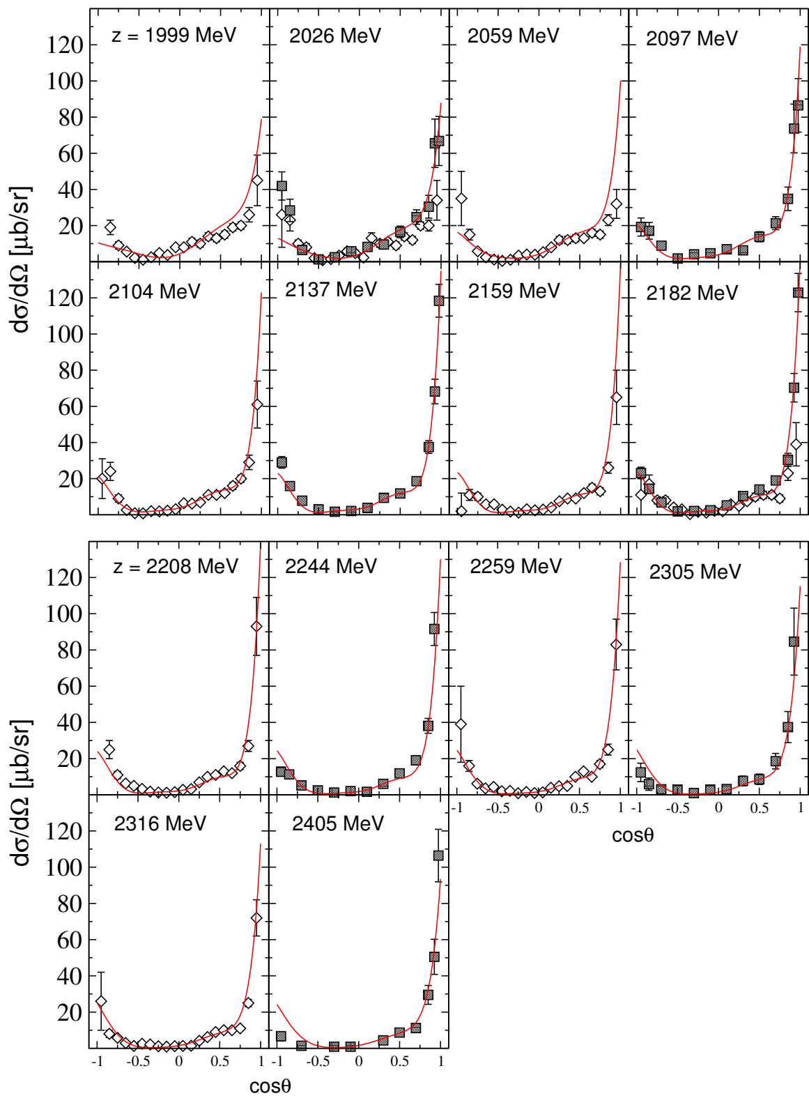
Figure 10: Differential cross section [3/3] of the reaction \pi^- p \rightarrow K^0 \Lambda . Data: c.f. Fig. 8.
