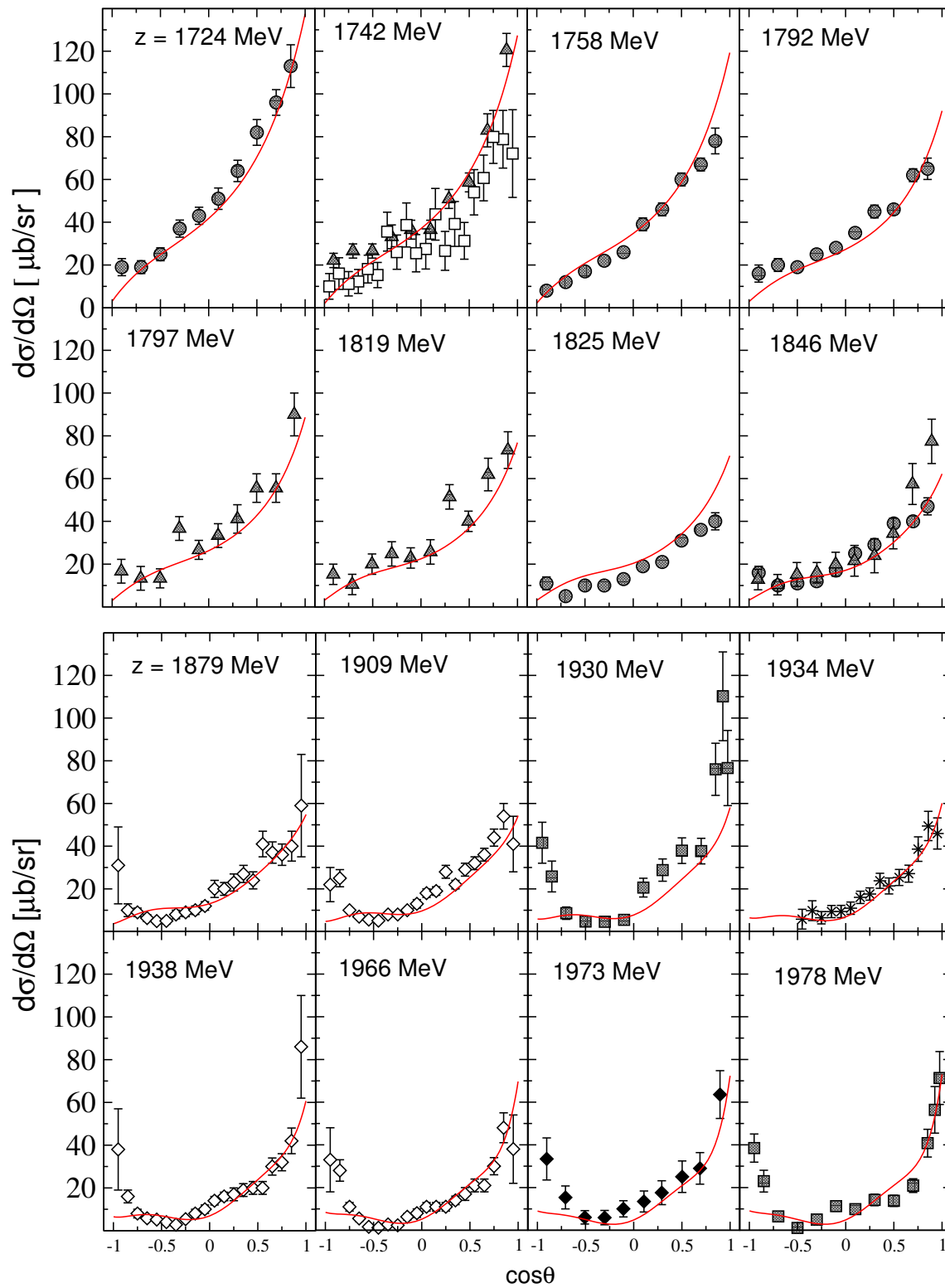
Figure 9: Differential cross section [2/3] of the reaction \pi^- p \rightarrow K^0 \Lambda . Data: c.f. Fig. 8.
