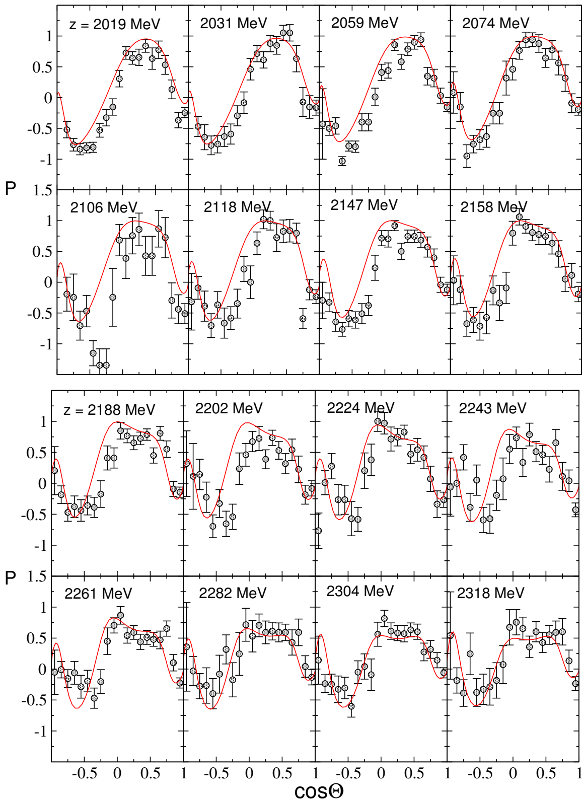
Figure 24: Polarization [2/2] of the reaction \pi^+p \rightarrow K^+\Sigma^+ . Data: Ref. [35].
