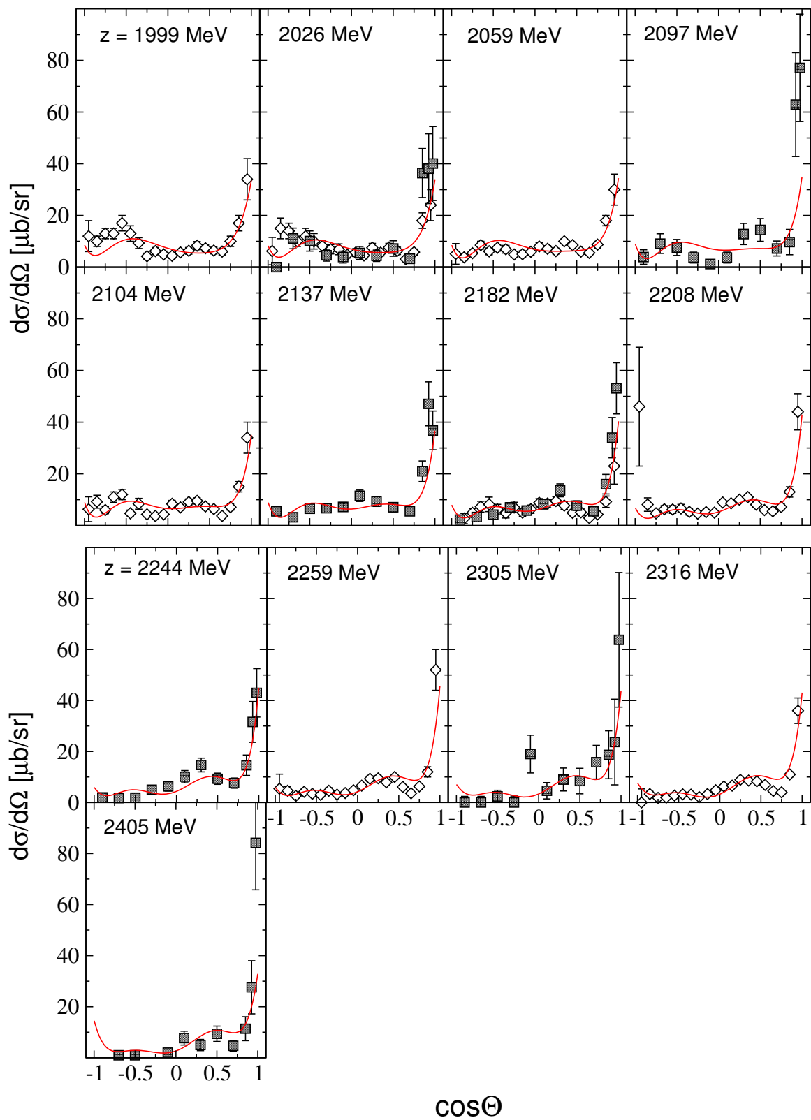
Figure 16: Differential cross section [2/2] of the reaction \pi^- p \rightarrow K^0 \Sigma^0 . Data: c.f. Fig. 15.
