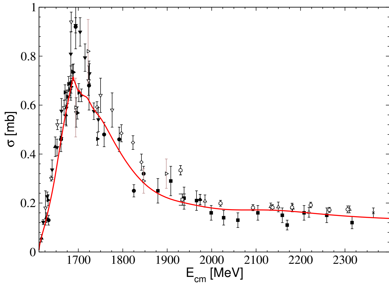
Figure 7: Total cross section of the reaction \pi^- p \rightarrow K^0 \Lambda . Data: filled circles from Ref. [12]; filled squares from Ref. [13]; empty diamonds from Ref. [14]; empty triangles up from Ref. [15]; filled triangles up from Ref. [16]; filled triangles down from Ref. [21]; empty triangles down from Ref. [22]; filled triangles right from Ref. [17]; empty triangles left from Ref. [23]; empty triangles right from Ref. [24]; empty squares from Ref. [18]; filled diamonds from Ref. [19]; stars from Ref. [25]; for empty circles and crosses see Ref. [26].
