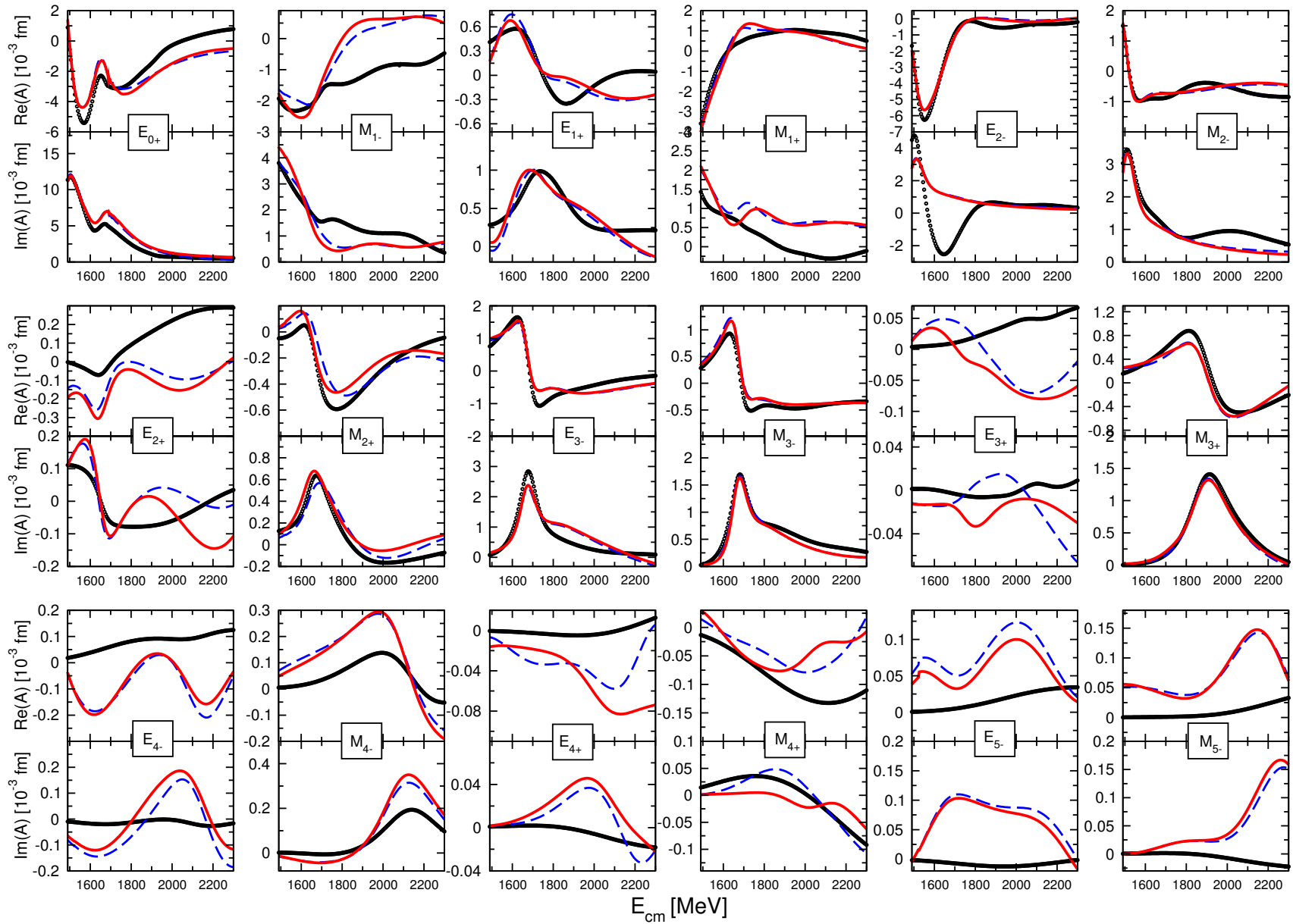
Figure 1: Blue lines: fit A Juelich2015, red lines: fit B Juelich2015. Black lines: Bonn-Gatchina solution BG 2014-2 (Eur. Phys. J. A 50 , 74 (2014)).
