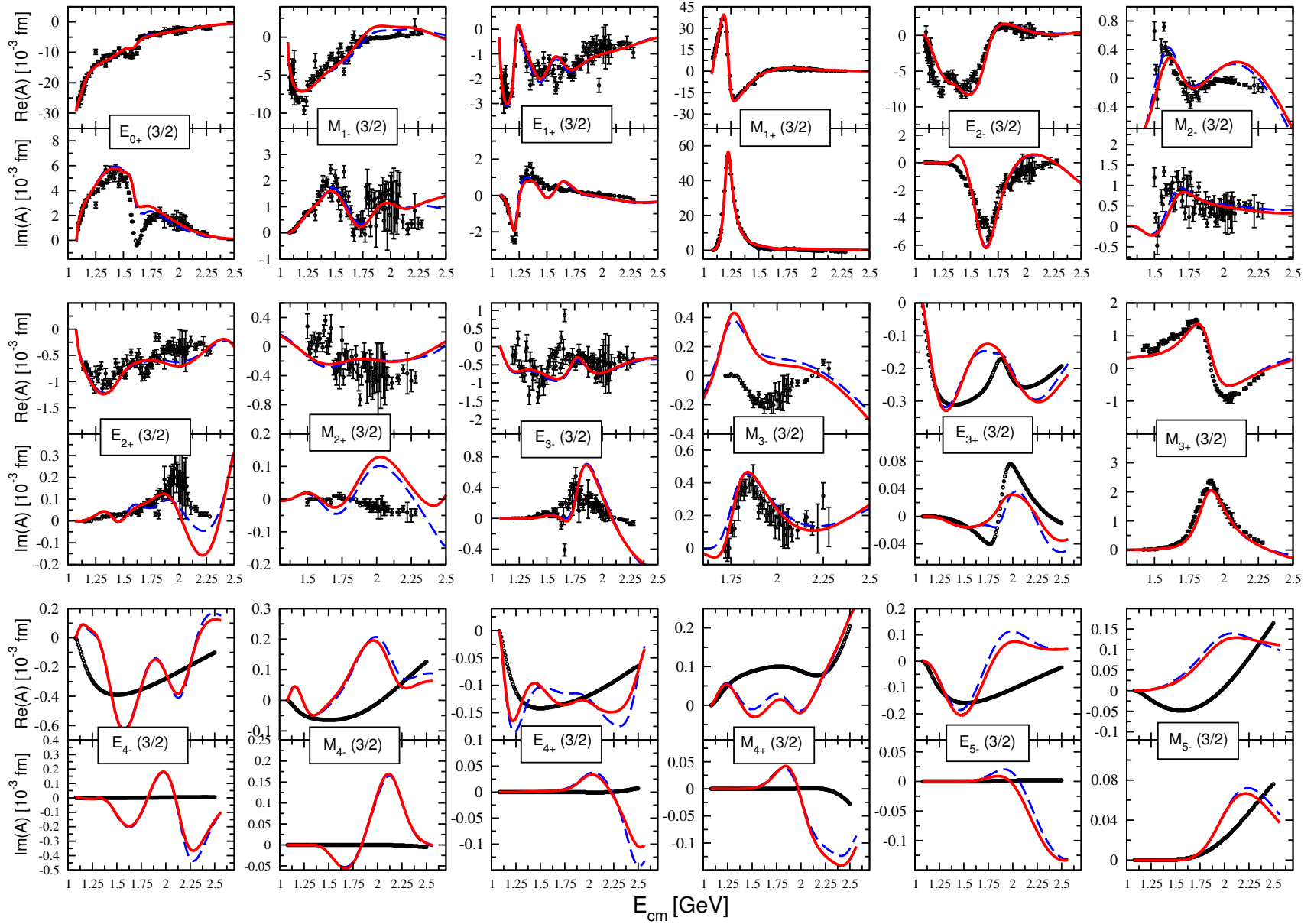
Figure 1: Blue lines: fit A Juelich2015, red lines: fit B Juelich2015. Black lines: GWU-SAID CM12 solution (Phys. Rev. C 86, 015202 (2012)).
