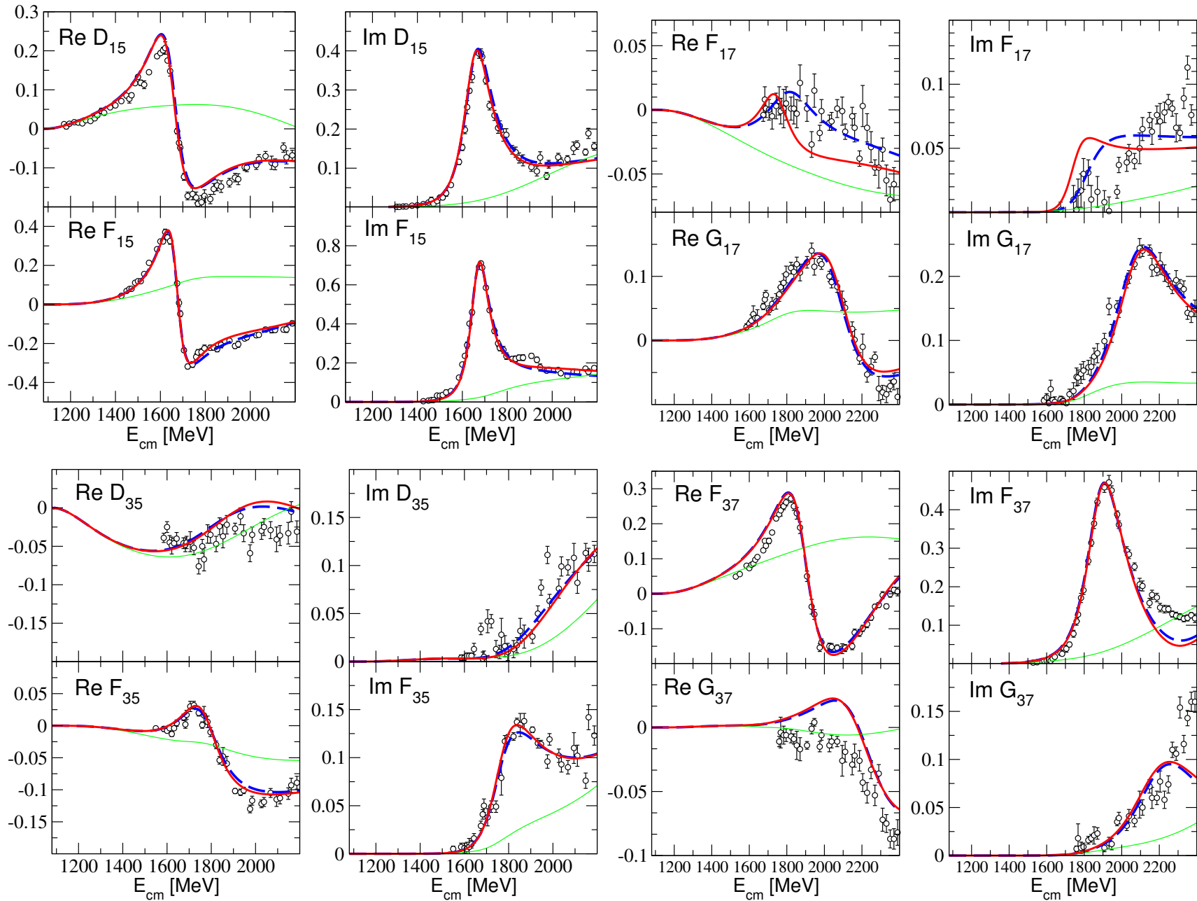
Figure 2: Jülich 2015, fit A: blue (dashed) line, fit B: red (solid) line, T^{\text{NP}} : green line. Points: GWU-SAID partial-wave analysis (Phys. Rev. C 74, 045205 (2006)).
