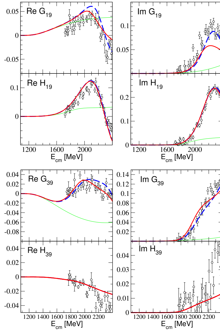
Figure 3: Jülich 2015, fit A: blue (dashed) line, fit B: red (solid) line, T^{\text{NP}} : green line. Points: GWU-SAID partial-wave analysis (Phys. Rev. C 74, 045205 (2006)).
