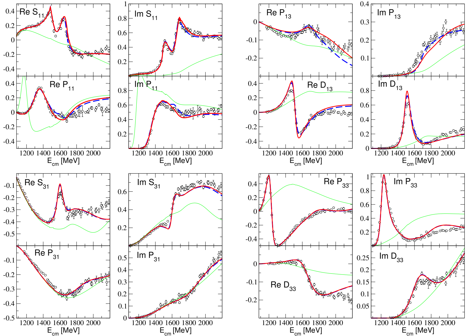
Figure 1: Jülich 2015, fit A: blue (dashed) line, fit B: red (solid) line, T^{\text{NP}} : green line. Points: GWU-SAID partial-wave analysis (Phys. Rev. C 74, 045205 (2006)).
