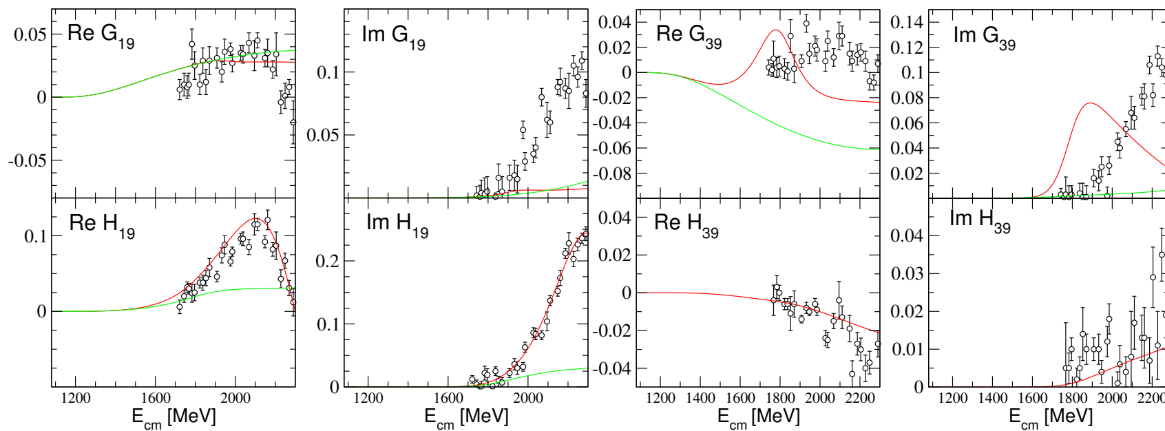
Figure 3: JüBo2017: red (solid) line, T^{\text{NP}} : green line. Points: GWU-SAID WI08 solution (Phys. Rev. C 86, 035202 (2012)).
