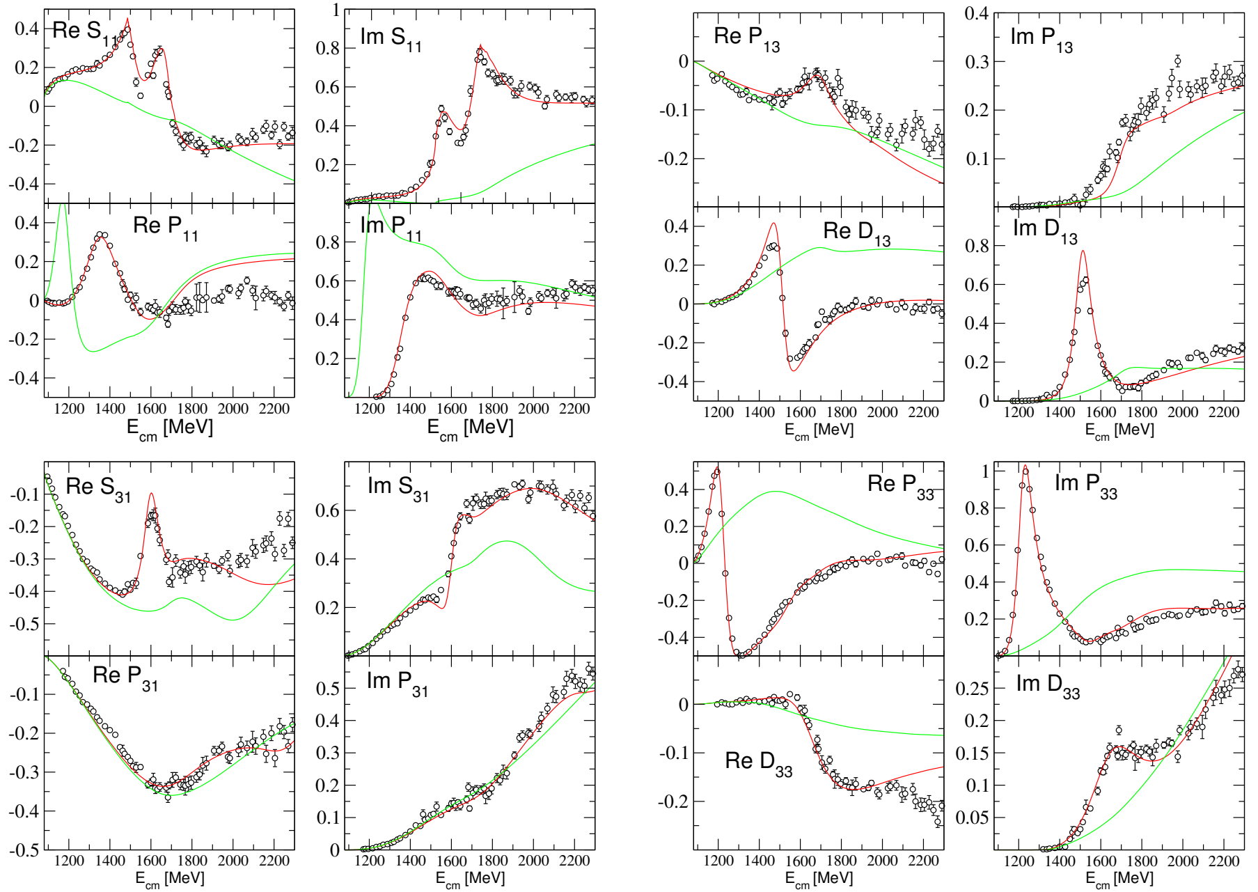
Figure 1: JüBo2017: red (solid) line, T^{\text{NP}} : green line. Points: GWU-SAID WI08 solution (Phys. Rev. C 86, 035202 (2012)).
