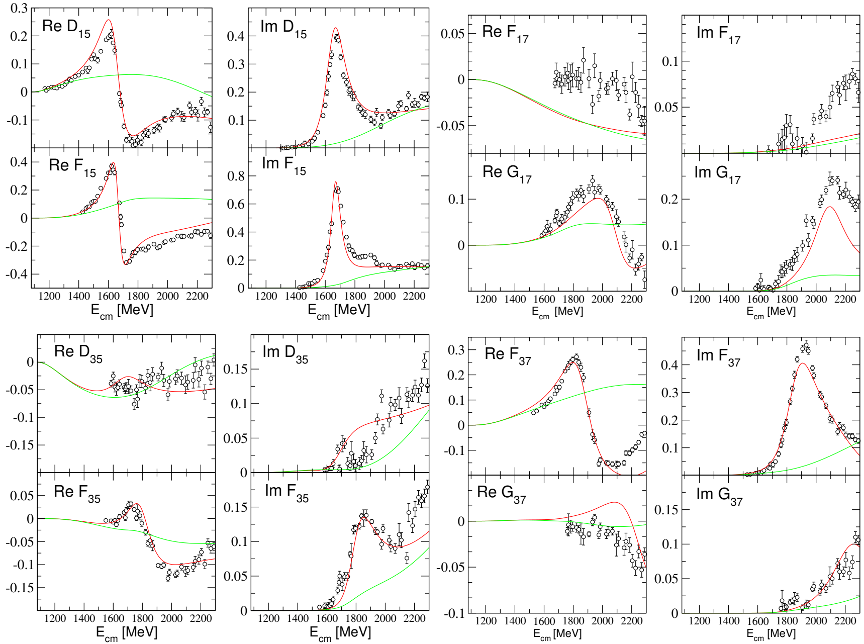
Figure 2: JüBo2017: red (solid) line, T^{\text{NP}} : green line. Points: GWU-SAID WI08 solution (Phys. Rev. C 86, 035202 (2012)).
