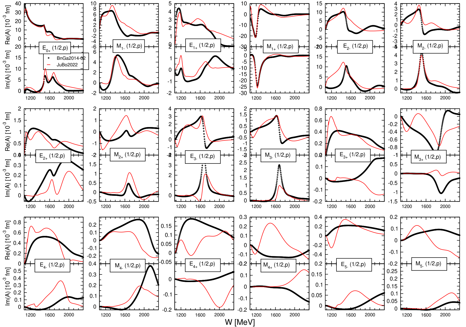
Figure 1: (Solid) red lines: JüBo2022. (Dashed) black lines: Bonn-Gatchina solution BG 2014-2 (Eur. Phys. J. A 50 , 74 (2014)).
