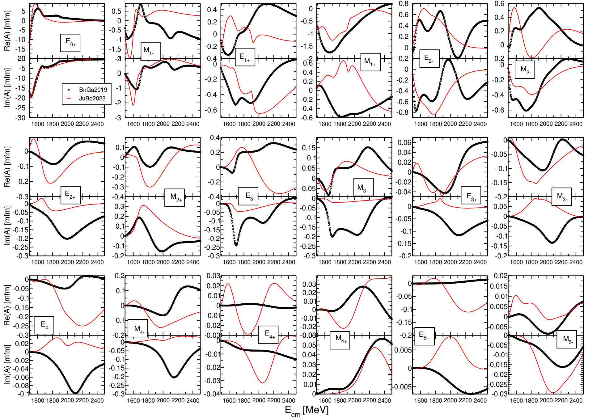
Figure 1: (Solid) red lines: JüBo2022. (Dashed) black lines: Bonn-Gatchina solution BG 2019 (Phys. Lett. B 803, 135323 (2020)).
