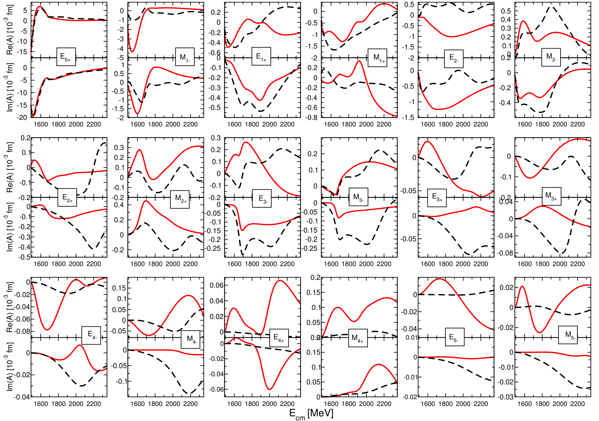
Figure 1: (Solid) red lines: JüBo2017. (Dashed) black lines: Bonn-Gatchina solution BG 2014-2 (Eur. Phys. J. A 50 , 74 (2014)).
