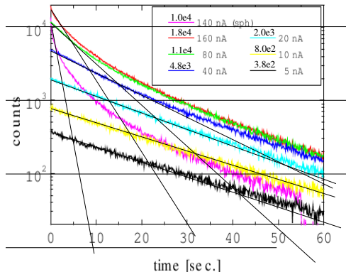
Figure 4: Stored ELISA beam current I(t) (expressed as “counts” C(t) ) surviving after time t , plotted vs t . The purpose for the straight lines superimposed on this graph (as preparation for the present report), was to determine the initial beam decay rate as a function of beam current. The results are plotted in Figure 5.
