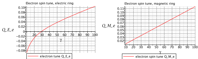
Figure 7: The “magic” value is \gamma_e \approx 30 , but this can be changed by a large factor by superimposing magnetic field on the electric bending field.
