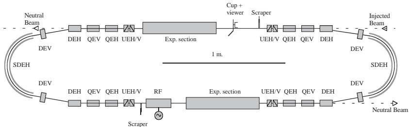
Figure 3: Layout of the ELISA low energy proton and ion storage ring, copied from Møller[2]
