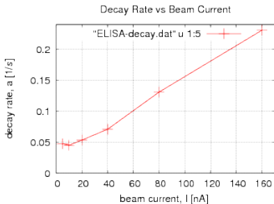
Figure 5: For beam current monitor counts C(t) , modeled as C(t) = C(0) e^{-a(I)t} , the initial decay rate a(I) is plotted as a function of stored current I . Procedure for obtaining this data is explained in the caption to Figure 4. For small beam currents the decay rate is roughly what is expected from scattering from residual vacuum chamber particles. It is the rapid increase in decay rate with increasing beam current that needs to be understood, and rectified, before an optimistic feasibility study for an eventual proton storage ring EDM measurement can be produced.
