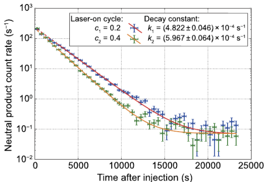
Figure 6: Beam survival plot for the Heidelberg CSR ring. This beam survival is at quite low beam current. Estimated parameters are given in the table shown previously..
