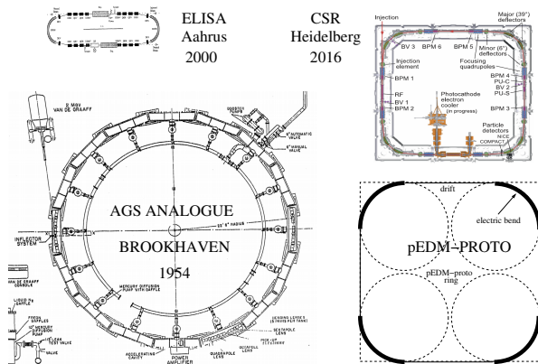
Figure 2: Layouts (all to more-or-less the same scale) of storage rings that can be viewed as prototypes for an eventual, all-electric, proton EDM storage ring, including, as well, a probably-undersized (because required equipment for injection, polarimetry, RF, etc is not included) cartoon of the proposed pEDM-PROTO ring.
