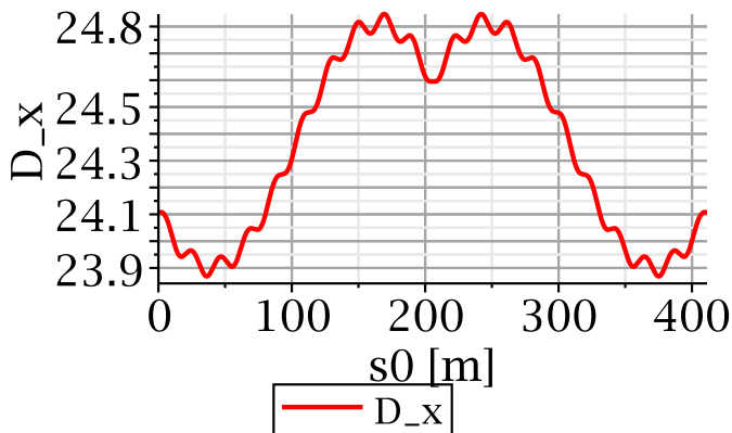
Figure 9: Outside dispersion function D^0(s) , plotted for full ring. For this case the total circumference is 411.3 m and the total drift length is 160.0 m.
