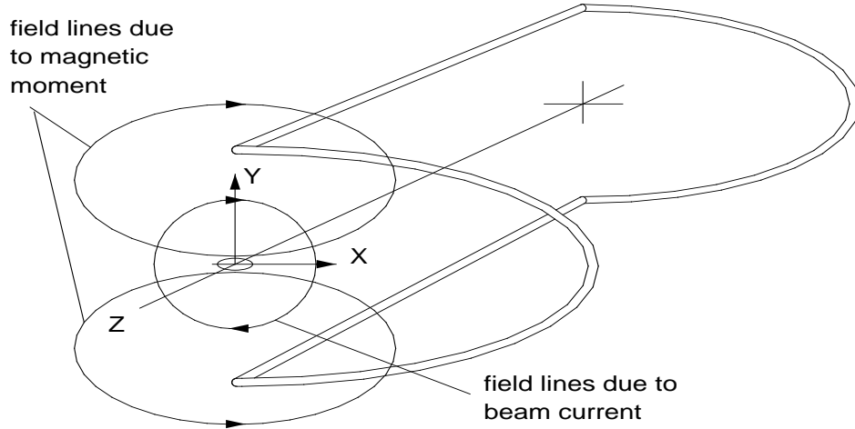
FIGURE 2. The Pickup Loop
