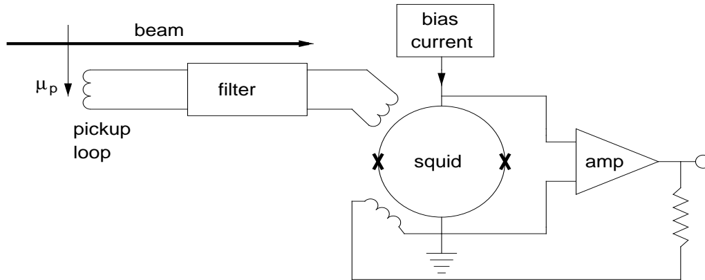
FIGURE 3. Block Diagram
