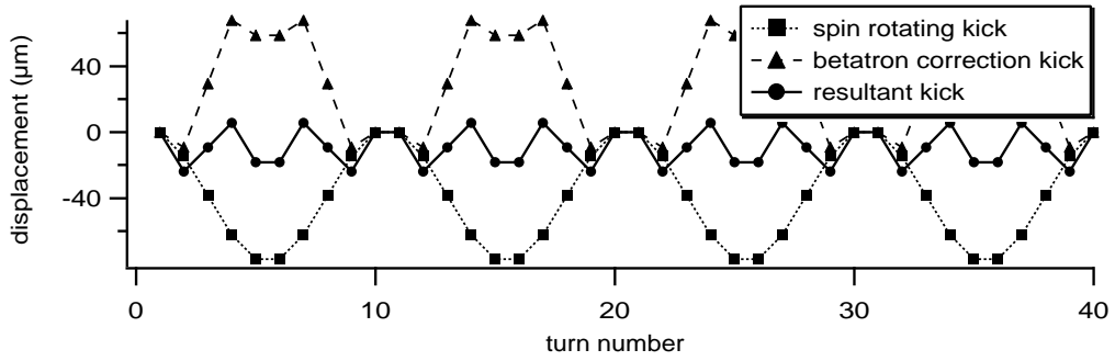
FIGURE 1. Beam Displacement due to Spin Flipping and Correction
