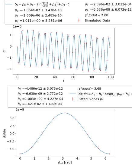
Figure 3: The upper graph shows the build-up of the angle \alpha = \arctan(P_V/P_H) in between vertical polarization P_V and horizontal polarization P_H as a function of revolutions t in COSY, using a RF-Wien filter scaling factor of A_0 = 1000 and a relative RF-Wien filter phase of \phi_{rel} = 2\pi . The fit parameter p_4 indicates the vertical build-up. This fit parameter was simulated for a variety of relative phases and plotted against the different relative phases in the lower graph. The fit parameter h_1 of a cosine fit to these data shows the so-called EDM resonance strength \epsilon_{EDM} .
