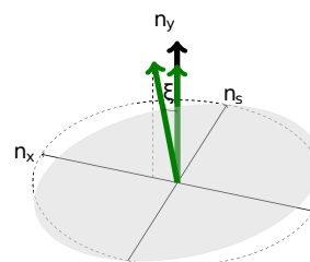
Figure 1: A permanent EDM of magnitude \eta tilts the invariant spin axis in horizontal direction n_x by the angle \xi . The longitudinal direction n_y is not affected by a permanent EDM.
