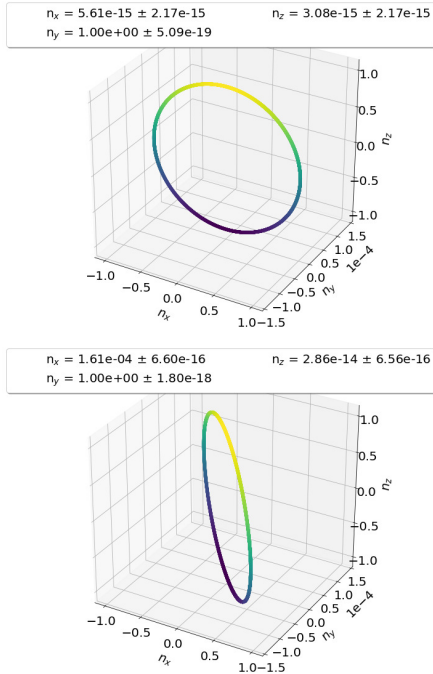
Figure 2: Spin precession plane simulated by tracking the reference particle for 10^4 revolutions in an idealized Bmad COSY model. The upper figure displays a simulation without an EDM signal, while the lower figure shows a simulation with an EDM signal of \eta = 10^{-4} included. The invariant spin axis \langle \vec{n} \rangle is the vector perpendicular to this plane. Its orientation is displayed in the legend.
