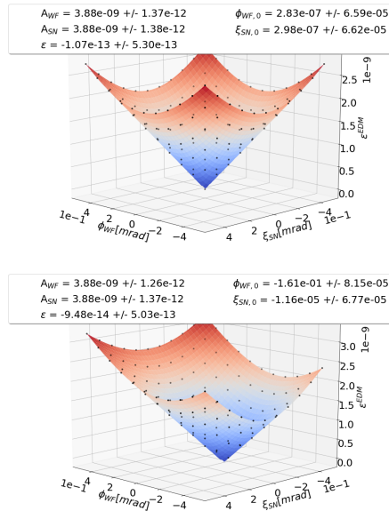
Figure 4: The upper graph shows a simulated resonance map without an EDM contribution, while the lower graph shows a simulated resonance map with an EDM signal of \eta = 10^{-4} . The x- and y-axis indicate the RF-Wien filter rotation and the solenoid strength, while the z-axis shows the EDM resonance strength. The legend shows the fit parameter when fitting Eq. (5) to the simulated data.
