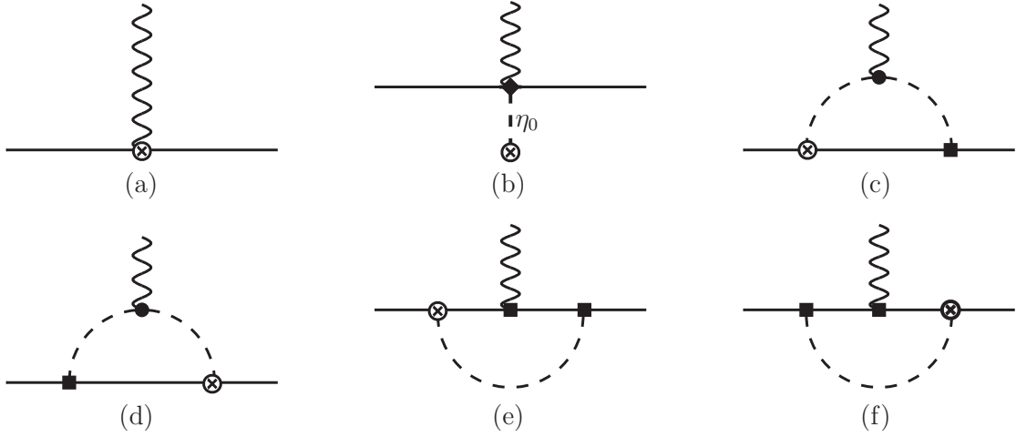
Figure 1. Feynman diagrams contributing to the baryon EDFs up to next-to-leading order, where \otimes denotes a CP violating vertex, black dots represent the second order mesonic vertices, filled squares and diamonds are the first and second order baryonic vertices, respectively.
