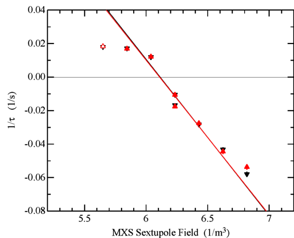
FIG. 16. Same as Fig. 15 but for wide beam scan 2, shown as a function of S ( G is zero). This is a subset of the data shown in Fig. 14.
