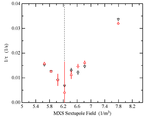
FIG. 20. Measurements made with the long beam of 1/\tau as a function of the S sextupole field (Scan 2). The G field is zero. The optimum field value is indicated by a dashed line.
