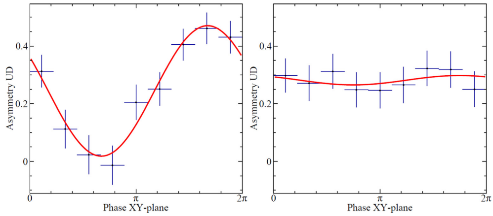
Fig. 3. Measurements of the up-down polarimeter asymmetry for a set of 9 directional bins during a 1-second time interval with horizontal polarization in the COSY ring. The two panels contain examples of a large and a small IPP. The red curve shows the best fit of a sinusoidal curve through these data. Its magnitude is proportional to the size of the IPP. The offset of the sine curve from zero arises from a geometrical misalignment of the polarimeter relative to the beam direction and does not affect the magnitude of the sine curve.
