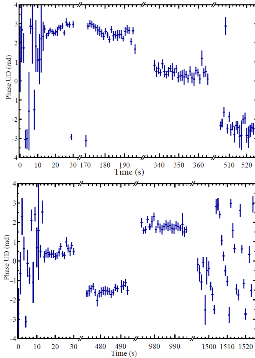
Fig. 4. (upper panel) Example of up-down phase data for one cycle in run 5021. (lower panel) Example of the up-down phase data from run 5039 for a cycle that was discarded from the analysis. Parts of the time axis without usable data have been removed. See text for more details.
