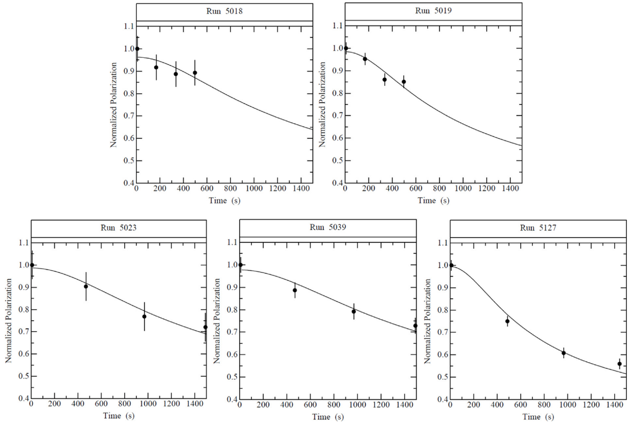
Fig. 6. Measurements of the IPP as a function of time. The top row shows runs 5018 and 5019, both of which had the shorter (564 s) data observation length. The second row shows measurements of the IPP for runs 5023, 5039, and 5127 where the longer observation time was applied. In all five cases, electron cooling was operating throughout the data acquisition period.
