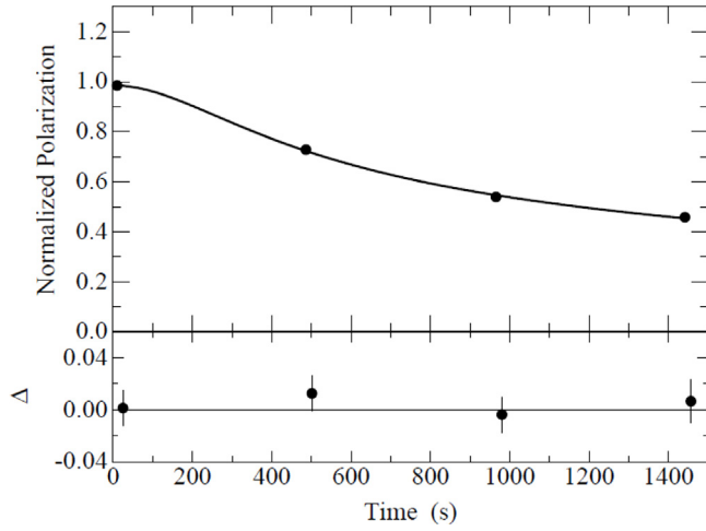
Fig. 1. Measurements of the normalized horizontal polarization as a function of time in the beam store along with a fitted curve used to estimate the polarization lifetime. The data is normalized to the vertical polarization of the beam before it was rotated into the ring plane. The curve represents the polarization of a Gaussian distribution of spin tunes as it evolves in time. The lower panel shows the residuals of the fit. Source: Taken from Ref. [3].
