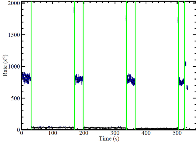
Fig. 2. Example of the up detector rate in a single machine cycle as a function of the time in the cycle. The origin of the horizontal axis corresponds to the beginning of the first extraction period; the initial part of the cycle devoted to beam preparation is not shown. The measurements are from run 5021. The vertical lines mark the limits of the data chosen for analysis. A spike in the rate leading to a high rate point always occurs whenever the white noise extraction is first turned on.
