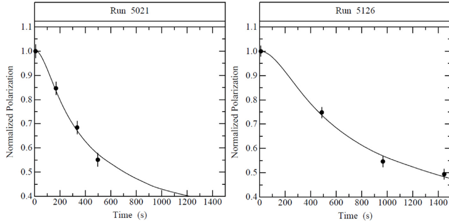
Fig. 5. Measurements of the normalized IPP as a function of time for runs 5021 and 5126. Both runs had only electron pre-cooling.
