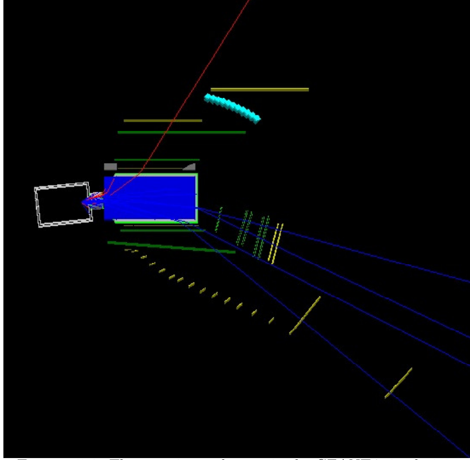
FIGURE 5.1: The experimental setup in the GEANT4 simulation.
