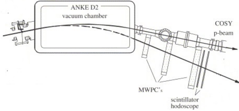
FIGURE 3.6: The top view of forward detection system.
