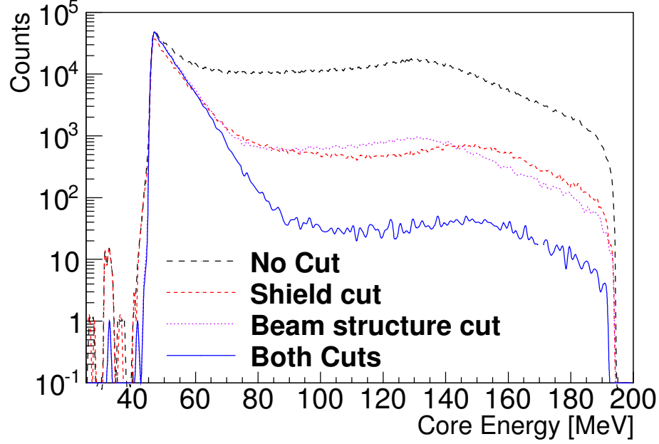
FIGURE B.4: (Color online) {}^3\text{He} run data in one NaI detector at 40^\circ . Blac line: no cut applied. Red line: only an anti-coincidence-shield cut applied. Magenta line: a cut of beam-time-stucture applied. Blue line: with both cuts [202].
