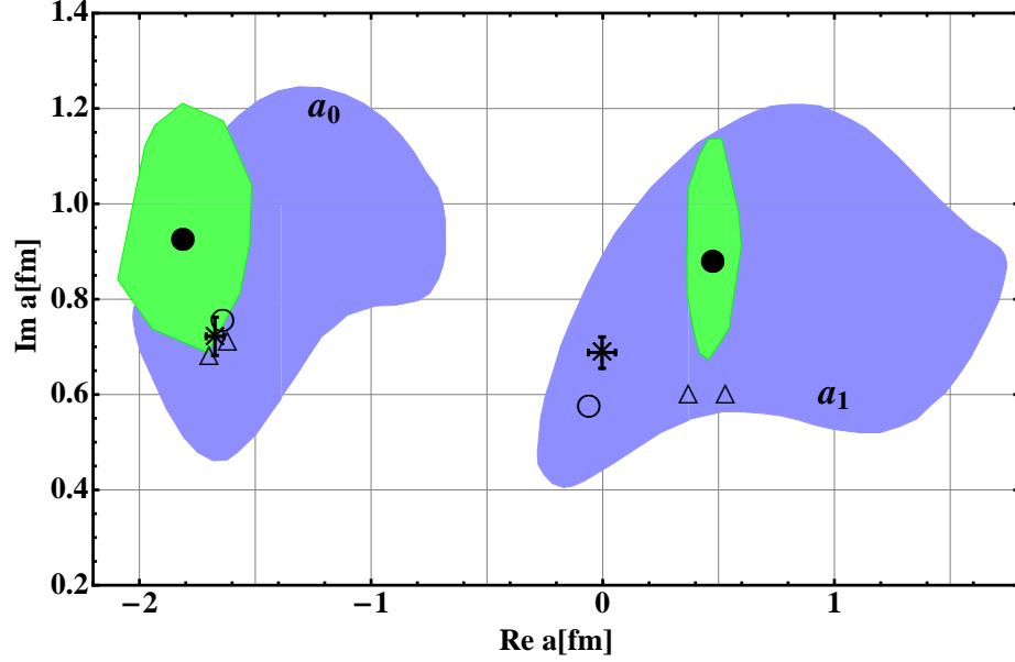
FIGURE 6.10: Real and imaginary part of isospin 0 and 1 KN \rightarrow KN scattering lengths. The light shaded (green) areas correspond to the 1\sigma region of our approach around the central value (full circles). The darker (blue) areas correspond to the 1\sigma region around central value (empty circle) from Ref. [179]. the cross and empty triangles denote older experimental values from [180] and [181], respectively.
