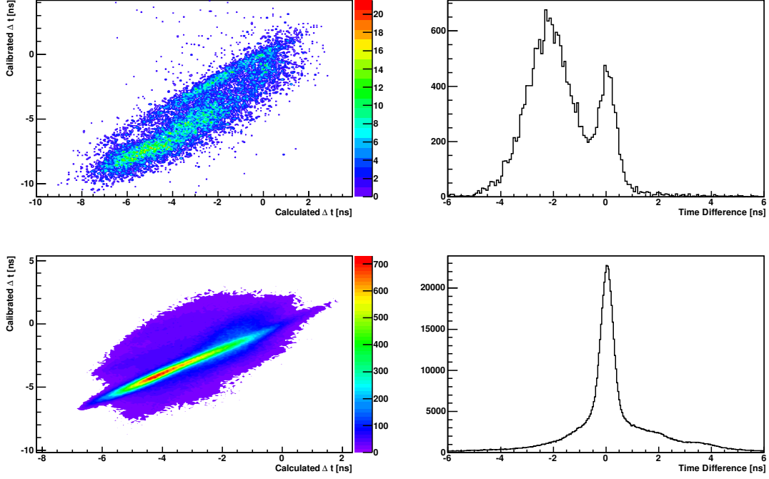
FIGURE 4.9: The left column shows: the TOF differences between the STOP counter in the negative as well as in the forward detector system with respect to the positive STOP counters versus TOF calculated using momentum information under the assumption that the detected particles are K^+K^- and K^+p . The right column shows its projection where clear separation between this pair can be performed.
