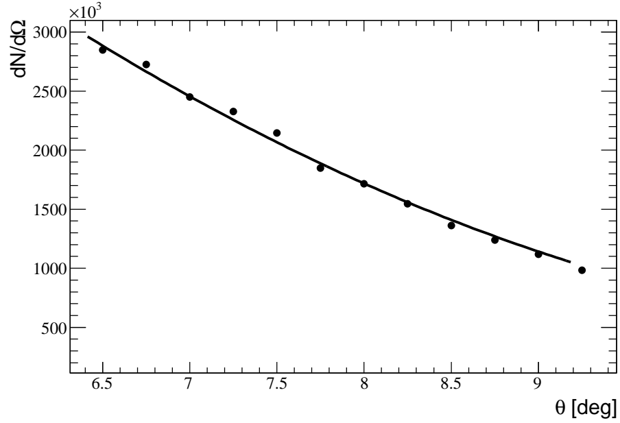
FIGURE 4.20: The events distribution for pp elastic scattering at T_p = 2.57 GeV. The points are experimental data and the cure is the prediction from the SAID solution multiplied by luminosity.
