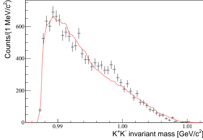
FIGURE 5.4: (Color online) The raw K^+K^- invariant mass distribution at \varepsilon = 23.9 MeV, \text{IM}_{K^+K^-} (points), is compared with the distribution of events obtained in a Monte Carlo simulation (curve). The error bars indicate only the statistical uncertainties.
