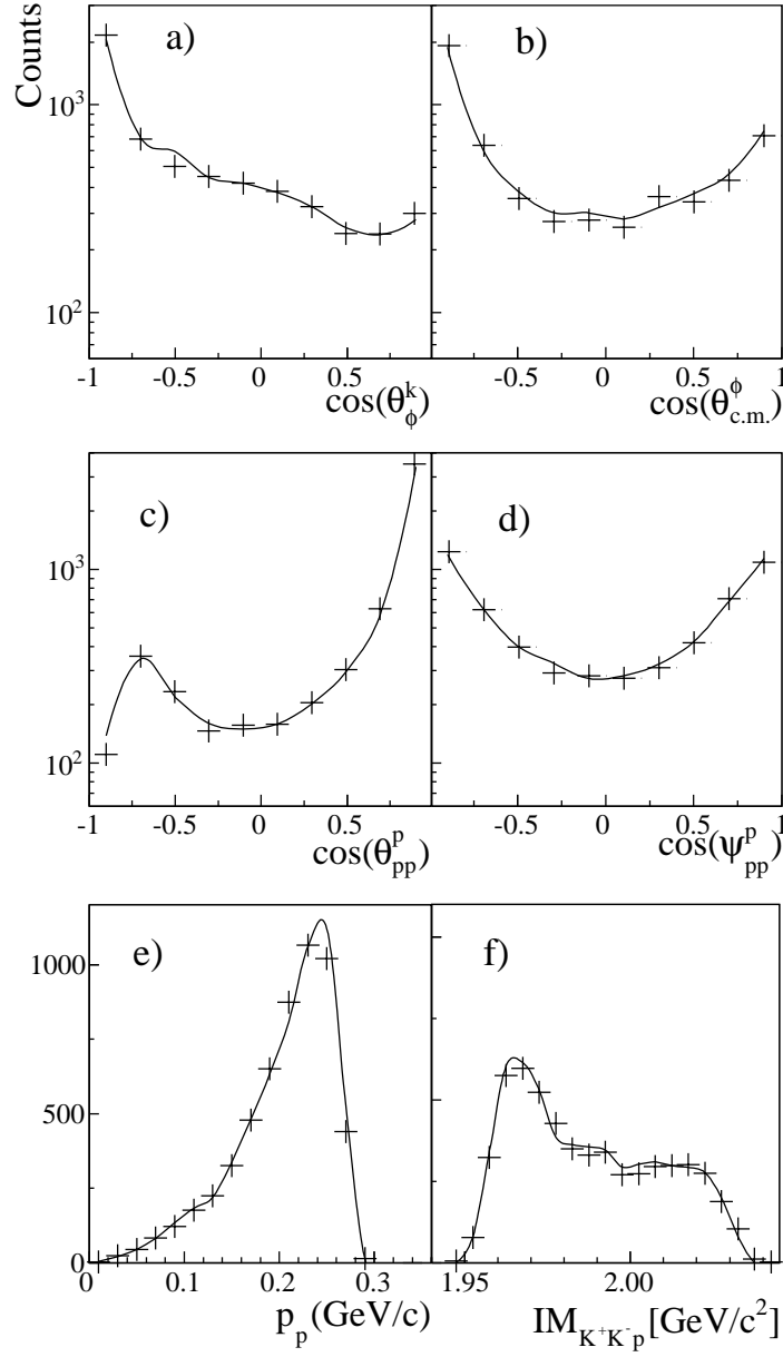
FIGURE 5.7: The differential distributions of yields in the \phi region ( 1.01 \text{ GeV}/c^2 < \text{IM}_{K^+K^-} < 1.03 \text{ GeV}/c^2 ) for the pp \rightarrow ppK^+K^- reaction at T_p = 2.83 \text{ GeV} , where the points are experimental data and the curves represent simulations. The notations for the six panels are the same as those in Fig. 5.5.
