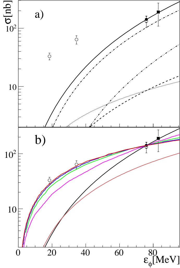
FIGURE 6.15: Total cross section for the pp \rightarrow pp\phi reaction as a function of excess energy \varepsilon_\phi . The present result (solid circle) is shown together with experimental data taken from DISTO [47] (solid square) and previous ANKE measurements [48] (open circles). (a) The data are compared to the black solid curve derived using Eq. with the parameters taken from Table. The individual contributions from the Ss (dotted curve), Sp (dashed curve), Ps (dashed-dotted curve), and Pp (double dotted-dashed) are normalized to their predicted values at 76 MeV. (b) The predictions of Tsushima and Nakayama [36] (magenta), scaled to pass through the 76 MeV point, underestimate the low energy data. Also shown are the predictions of Kaptari and Kampfer [182] (green), which are very similar to those of three-body phase-space with the inclusion of the pp FSI, the results within a resonance model Xie [1] (blue), and a one-pion-exchange model of Sibirtsev [52] (brown), and this plus exotic baryons [22] (red).
