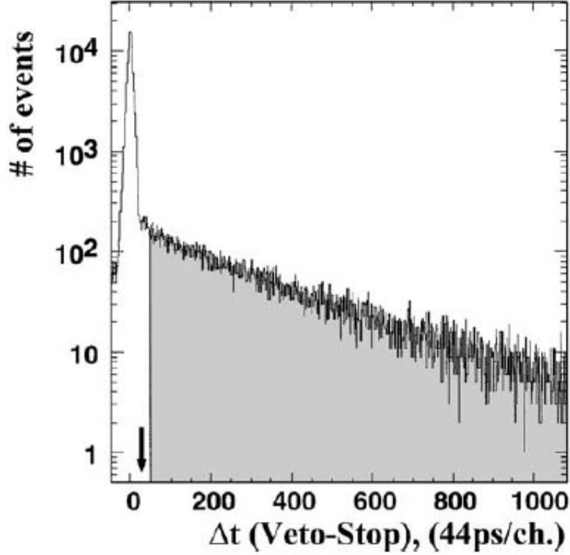
FIGURE 4.3: Time difference between detection of particles in veto and stop counters of telescope 13. The arrow shows the cut used during the measurements where the off-line cut is indicated by the shaded area.
