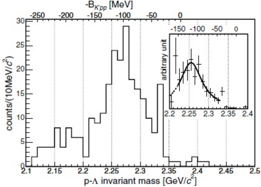
FIGURE 2.8: \Lambda p invariant mass spectrum from FINUDA experiment [128].
