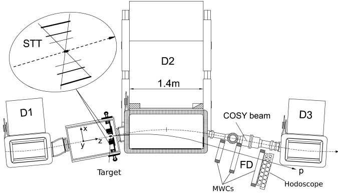
Figure 1: The ANKE spectrometer setup (top view), showing the positions of the hydrogen cluster-jet target, the silicon tracking telescopes (STT), and the forward detector (FD).
