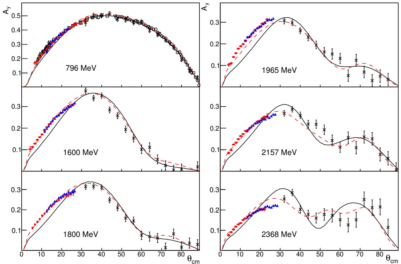
Figure 3: (Color online) Comparison of the ANKE measurements of the proton analysing power in pp elastic scattering using the STT (red filled circles) and FD (blue filled triangles) systems with the curves corresponding to the SAID SP07 (solid black line) and the revised fit (dashed red) solutions [1]. Only statistical errors are shown so that the systematic uncertainties arising, for example, from the calibration of the EDDA polarimeter have not been included. Also shown are selected results from EDDA (black crosses) [3] at the energies different by no more than 7 MeV and, at 796 MeV, LAMPF [17, 18, 19], and SATURNE [20] (black open symbols). It should be noted that the EDDA data were taken over a continuous ramp [3] and, if continuity in energy were imposed, many of their statistical fluctuations would be diminished.
