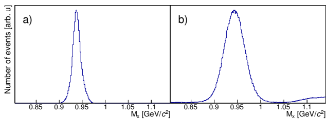
Figure 2: Missing-mass M_X(pp \rightarrow pX) spectra obtained for a beam energy of 1.6 GeV showing the clear proton peak when detecting one proton in (a) the STT and (b) the FD.
