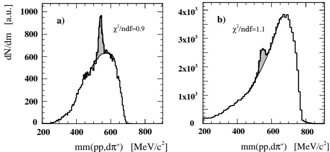
FIG. 6: Missing mass distribution mm(pp, d\pi^+) for the momentum ranges p_d = (1.4 - 1.6) GeV/c (a) and p_d = (1.6 - 2.8) GeV/c (b).
