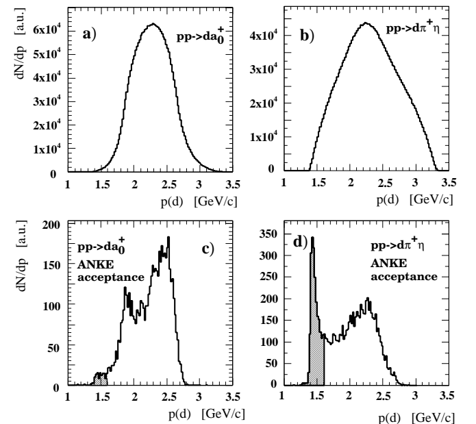
FIG. 4: Simulated acceptance for the deuteron momentum for the resonant (a,c) and the non-resonant (b,d) \pi^+\eta production. Upper row: the initial model distributions [29, 31–33]; lower row: momentum distributions within the ANKE acceptance.
