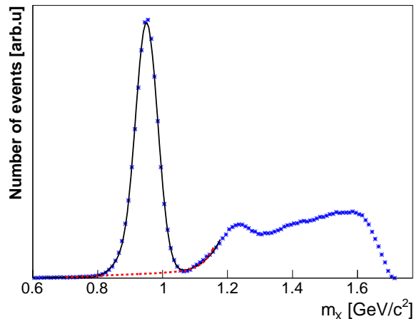
Fig. 4. Missing-mass M_X spectra obtained for the pd \rightarrow ppn reaction at a beam energy of 1800 MeV when detecting one proton in the right side STT and the other one in the FD. This distribution shows a clear neutron peak with little background, estimated by the straight (red) dashed line drawn from outside the peak region. It is possible that the start of the continuum reveals evidence for \Delta(1232) excitation. The solid (blue) curve is the Gaussian fit to the background-subtracted data in the neutron peak region.
