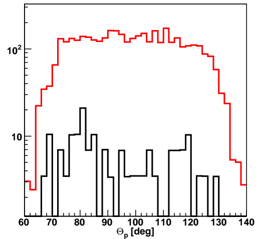
Fig. 5. The acceptance for the pd \rightarrow ppn_{\text{spec}} (black lines) and pd \rightarrow pnp_{\text{spec}} (red lines) reactions simulated within the framework of the incoherent “spectator” model at T_p = 800 MeV. A fast proton is detected in the FD and a slow one in the right-side STT at a laboratory angle \Theta_p .
