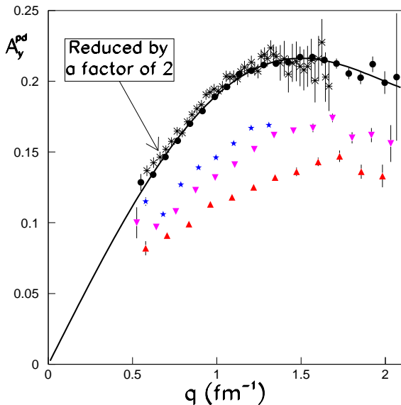
Fig. 3. The proton analyzing power A_y^{pd} in proton-deuteron elastic scattering as a function of the momentum transfer q in the centre-of-mass frame. ANKE data at 796 MeV are shown by closed (black) circles, at 1600 MeV by (blue) stars, at 1965 MeV by (magenta) inverted triangles, and at 2368 MeV by (red) triangles. Only statistical errors are shown and in general these are smaller than the symbol size. The fit of Eq. (1) to the ANKE data at 796 MeV is shown by the continuous curve. The LAMPF data at this energy are shown by (black) crosses [13]. In order to increase the visibility of the higher energy points, the results and curve at 796 MeV are reduced by a factor of two. The numerical values of the ANKE data are to be found in Table 2.
