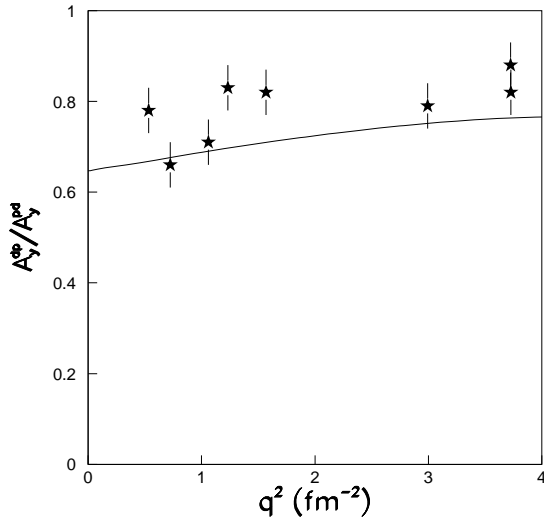
Fig. 8. The ratio between the vector analyzing power of the deuteron to that of the proton in \vec{p}d elastic scattering at 796 MeV per nucleon. The values of A_y^{dp} have been read with difficulty from a figure in Ref. [39] whereas those of A_y^{pp} were taken from the fit of Eq. (1) to the current data. The curve represents the results of an extended multiple scattering model using the formulae given in Ref. [42].
