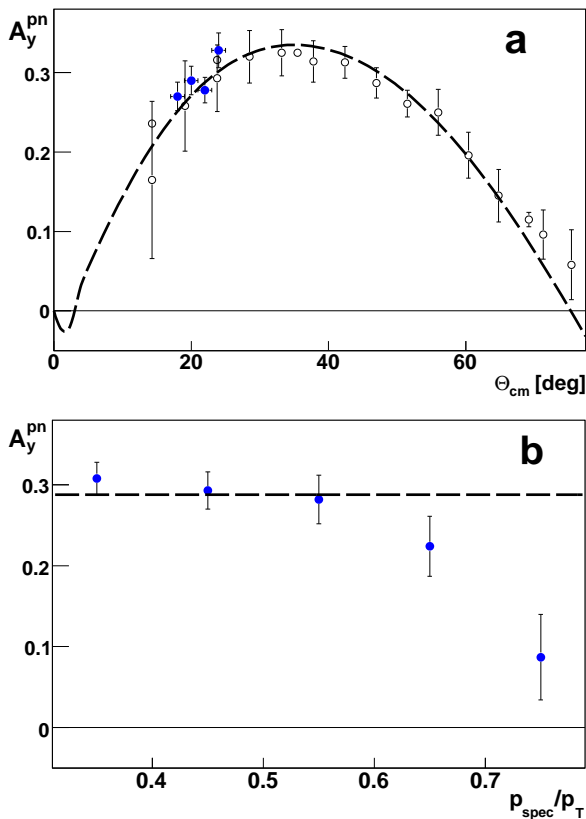
Fig. 6. Analyzing power A_y^{pn} in quasi-free \vec{p}n elastic scattering at T_p \approx 800 MeV. Panel (a): The open points are results from Ref. [31] as a function of the centre-of-mass scattering angle \Theta_{cm} . The blue solid points show results from the current experiment extracted, as discussed in the text, under conditions where p_{spec}/p_T < 0.5 and p_T > 200 MeV/c, where p_T is the laboratory momentum transfer. The predictions of the SAID SP07 partial wave solution [10] are shown by the dashed curve. Panel (b): The values of A_y^{pn} measured at ANKE for \Theta_{cm} = 22^\circ \pm 2^\circ as a function of the p_{spec}/p_T ratio. The dashed line indicates the SAID SP07 solution for A_y^{pn}(\Theta_{cm} = 22^\circ) [10].
