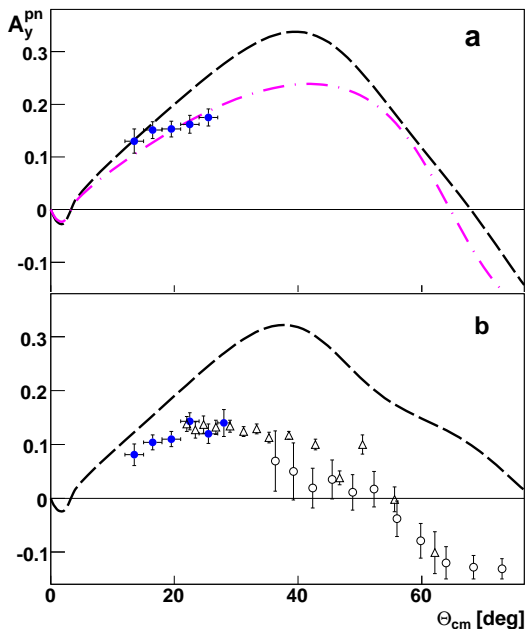
Fig. 7. A_y^{pn} of quasi-free \bar{p}n elastic scattering at (a) 1600 MeV and (b) 2200 MeV as function of the centre-of-mass scattering angle \Theta_{cm} . Solid (blue) points show the values obtained in the ANKE experiment whereas open (black) points are results taken from Ref. [32] (triangles) and Ref. [33] (circles). The magenta dot-dashed curve represents the new AD14 SAID solution at 1600 MeV [38], though it should be noted that this energy is outside the stated range of validity of this solution. The dashed (black) curves in both panels illustrate the previous SAID solution [10], though it must be stressed that this also has limited validity above 1300 MeV.
