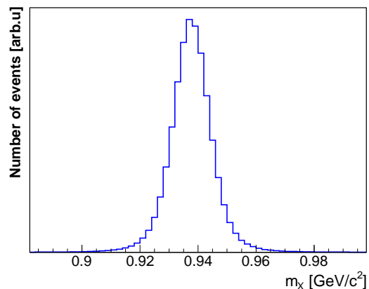
Fig. 2. The missing-mass distribution for the pd \rightarrow dX reaction at T_p = 796 MeV where the slow deuteron was detected in the left-side STT. Since no information from the forward detector was used here, the widths of the distributions are almost independent of beam energy. For the same reason, the results obtained from the two STT yield, of course, indistinguishable missing-mass distributions.
