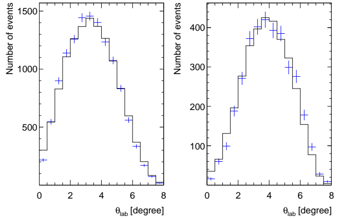
Fig. 5. Simulated (solid histogram) and experimental angular distributions for the dp \rightarrow p_{sp}d\pi^0 reaction at T_d = 1.2 GeV. The left and right panels correspond to fast and slow deuterons, respectively.
