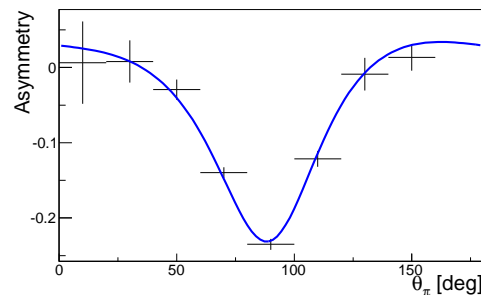
Fig. 2. Determination of the beam polarization, P_{\text{beam}} = 50 \pm 2\%
